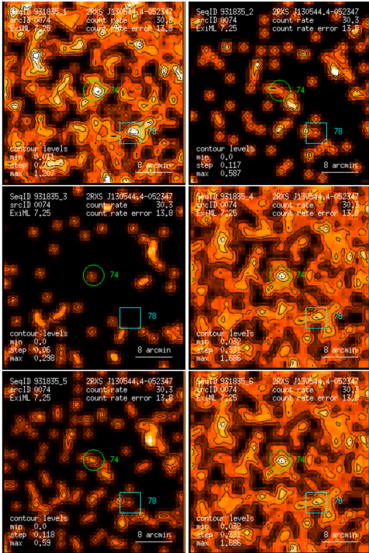
Figure 74: RASS 931835: detection 0074: band rate images, Gaussian filter: (1) PSPC channels 11 – 41, (2) 52 – 90, (3) 91 – 201, (4) 11 – 235, (5) 52 – 201, (6) 11 – 201. Broad band rates in counts/ks. Band rate contour levels in counts/ks/arcmin 2 .
