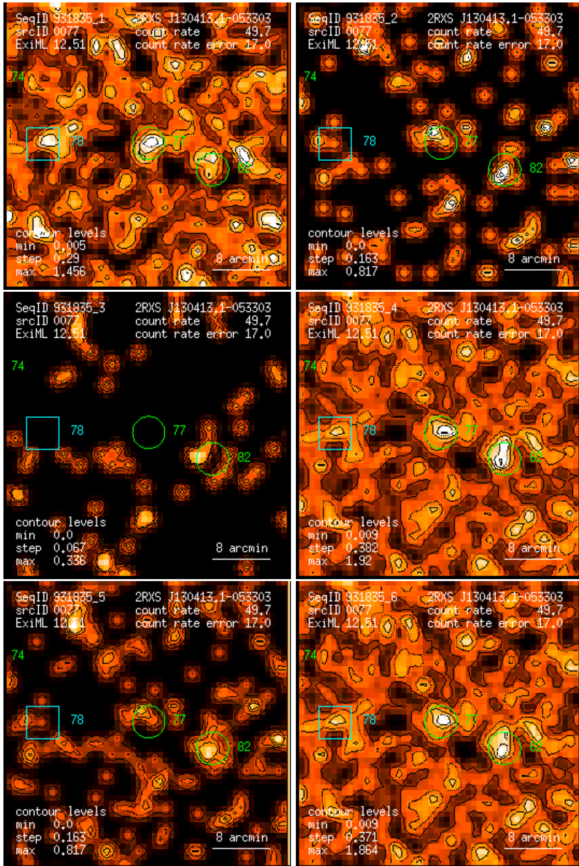
Figure 77: RASS 931835: detection 0077: band rate images, Gaussian filter: (1) PSPC channels 11 – 41, (2) 52 – 90, (3) 91 – 201, (4) 11 – 235, (5) 52 – 201, (6) 11 – 201. Broad band rates in counts/ks. Band rate contour levels in counts/ks/arcmin 2 .
