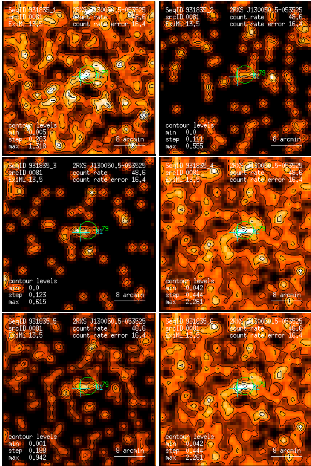
Figure 81: RASS 931835: detection 0081: band rate images, Gaussian filter: (1) PSPC channels 11 – 41, (2) 52 – 90, (3) 91 – 201, (4) 11 – 235, (5) 52 – 201, (6) 11 – 201. Broad band rates in counts/ks. Band rate contour levels in counts/ks/arcmin 2 .
