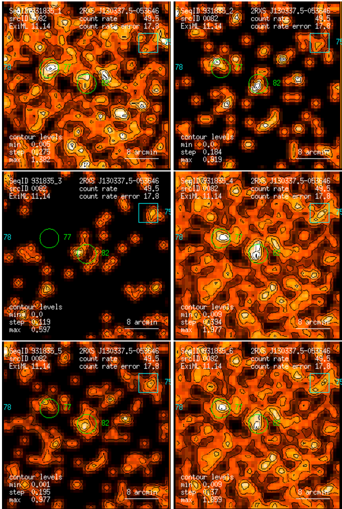
Figure 82: RASS 931835: detection 0082: band rate images, Gaussian filter: (1) PSPC channels 11 – 41, (2) 52 – 90, (3) 91 – 201, (4) 11 – 235, (5) 52 – 201, (6) 11 – 201. Broad band rates in counts/ks. Band rate contour levels in counts/ks/arcmin 2 .
