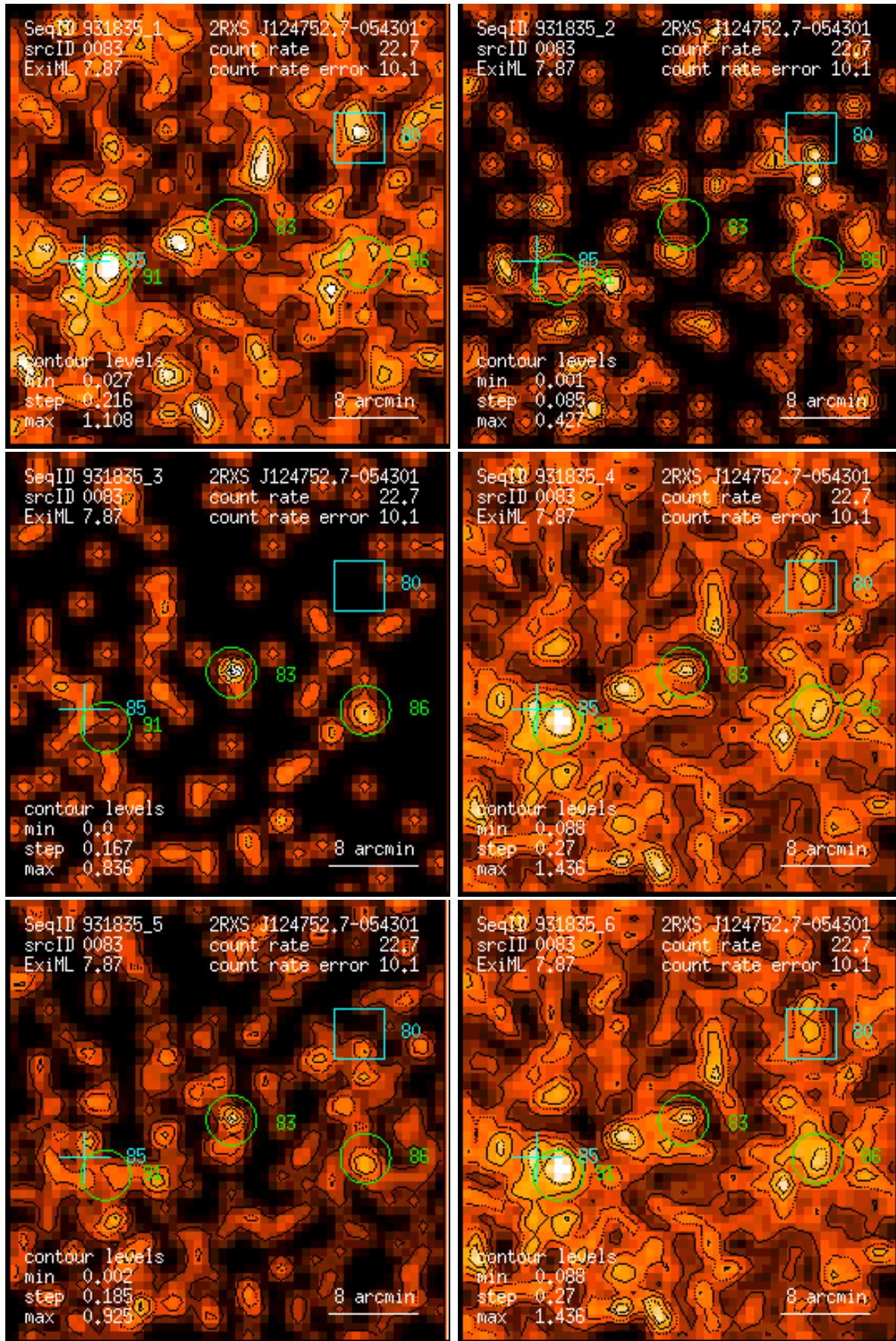
Figure 83: RASS 931835: detection 0083: band rate images, Gaussian filter: (1) PSPC channels 11 – 41, (2) 52 – 90, (3) 91 – 201, (4) 11 – 235, (5) 52 – 201, (6) 11 – 201. Broad band rates in counts/ks. Band rate contour levels in counts/ks/arcmin 2 .
