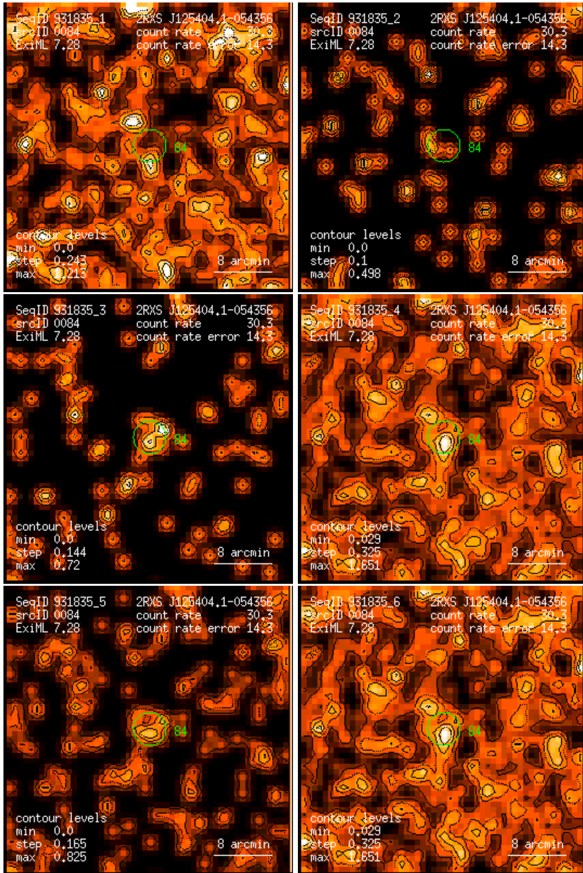
Figure 84: RASS 931835: detection 0084: band rate images, Gaussian filter: (1) PSPC channels 11 – 41, (2) 52 – 90, (3) 91 – 201, (4) 11 – 235, (5) 52 – 201, (6) 11 – 201. Broad band rates in counts/ks. Band rate contour levels in counts/ks/arcmin 2 .
