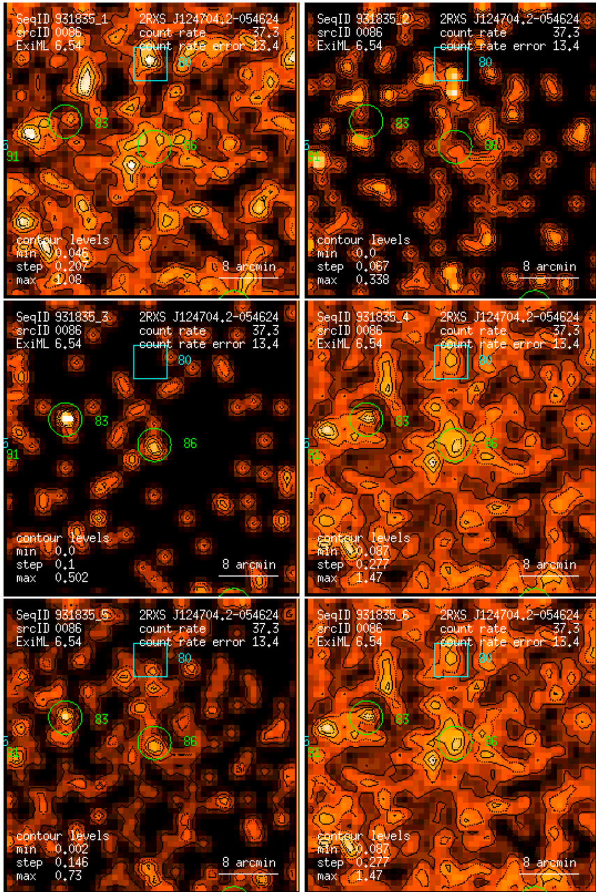
Figure 86: RASS 931835: detection 0086: band rate images, Gaussian filter: (1) PSPC channels 11 – 41, (2) 52 – 90, (3) 91 – 201, (4) 11 – 235, (5) 52 – 201, (6) 11 – 201. Broad band rates in counts/ks. Band rate contour levels in counts/ks/arcmin 2 .
