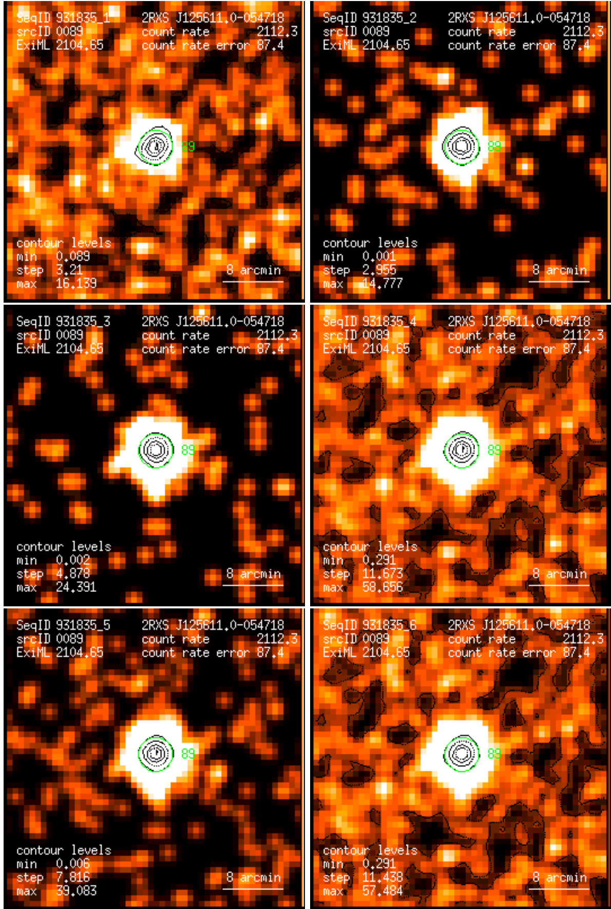
Figure 89: RASS 931835: detection 0089: band rate images, Gaussian filter: (1) PSPC channels 11 – 41, (2) 52 – 90, (3) 91 – 201, (4) 11 – 235, (5) 52 – 201, (6) 11 – 201. Broad band rates in counts/ks. Band rate contour levels in counts/ks/arcmin 2 .
