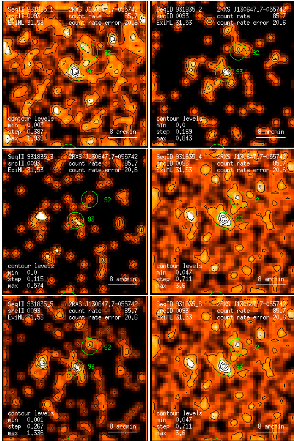
Figure 93: RASS 931835: detection 0093: band rate images, Gaussian filter: (1) PSPC channels 11 – 41, (2) 52 – 90, (3) 91 – 201, (4) 11 – 235, (5) 52 – 201, (6) 11 – 201. Broad band rates in counts/ks. Band rate contour levels in counts/ks/arcmin 2 .
