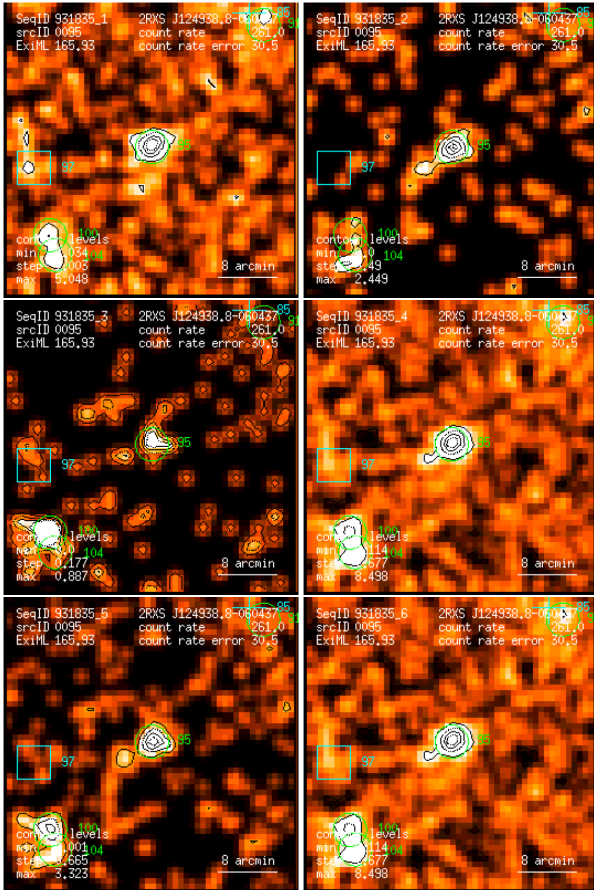
Figure 95: RASS 931835: detection 0095: band rate images, Gaussian filter: (1) PSPC channels 11 – 41, (2) 52 – 90, (3) 91 – 201, (4) 11 – 235, (5) 52 – 201, (6) 11 – 201. Broad band rates in counts/ks. Band rate contour levels in counts/ks/arcmin 2 .
