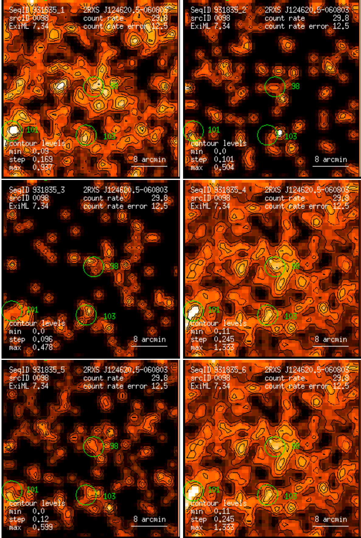
Figure 98: RASS 931835: detection 0098: band rate images, Gaussian filter: (1) PSPC channels 11 – 41, (2) 52 – 90, (3) 91 – 201, (4) 11 – 235, (5) 52 – 201, (6) 11 – 201. Broad band rates in counts/ks. Band rate contour levels in counts/ks/arcmin 2 .
