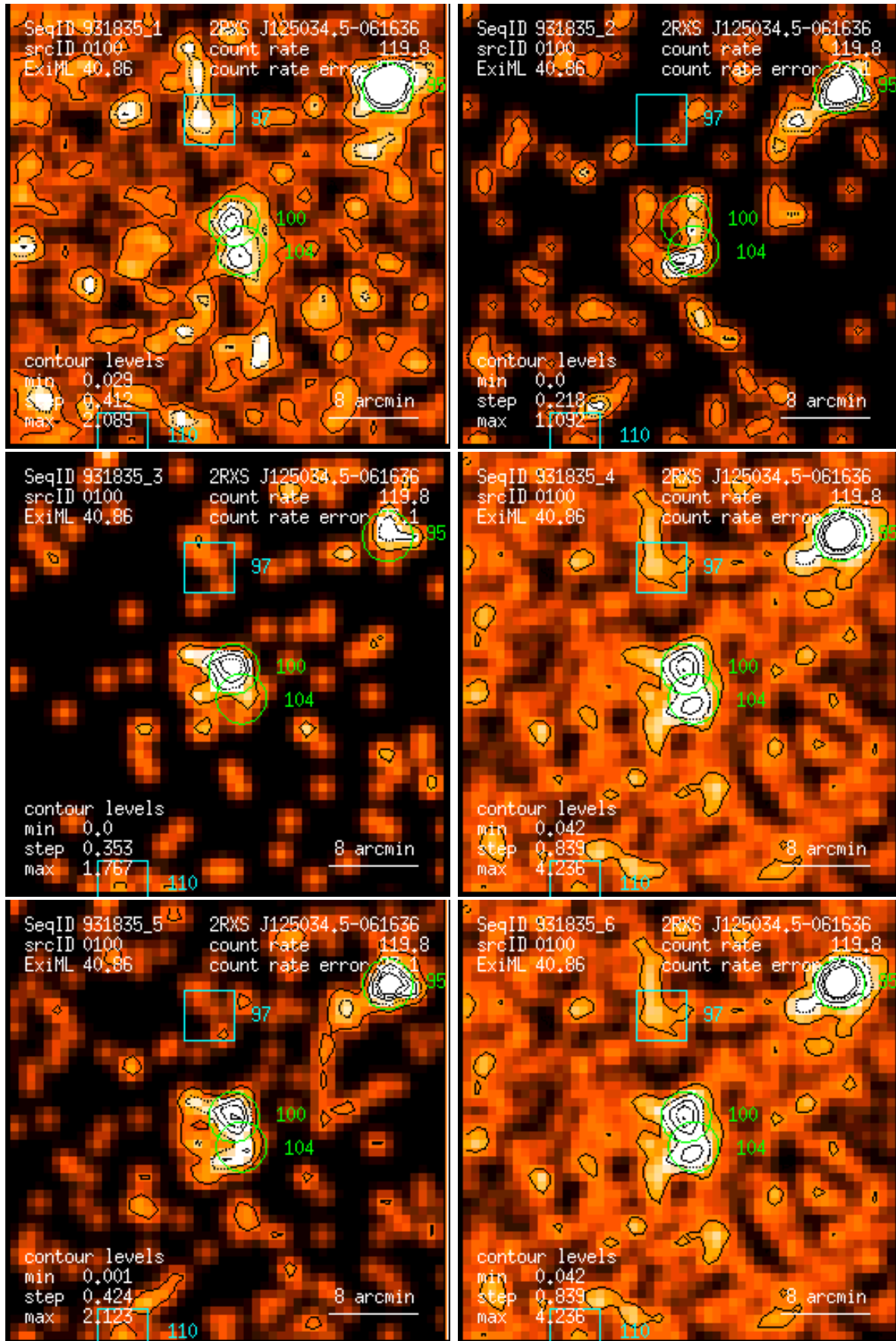
Figure 100: RASS 931835: detection 0100: band rate images, Gaussian filter: (1) PSPC channels 11 – 41, (2) 52 – 90, (3) 91 – 201, (4) 11 – 235, (5) 52 – 201, (6) 11 – 201. Broad band rates in counts/ks. Band rate contour levels in counts/ks/arcmin 2 .
