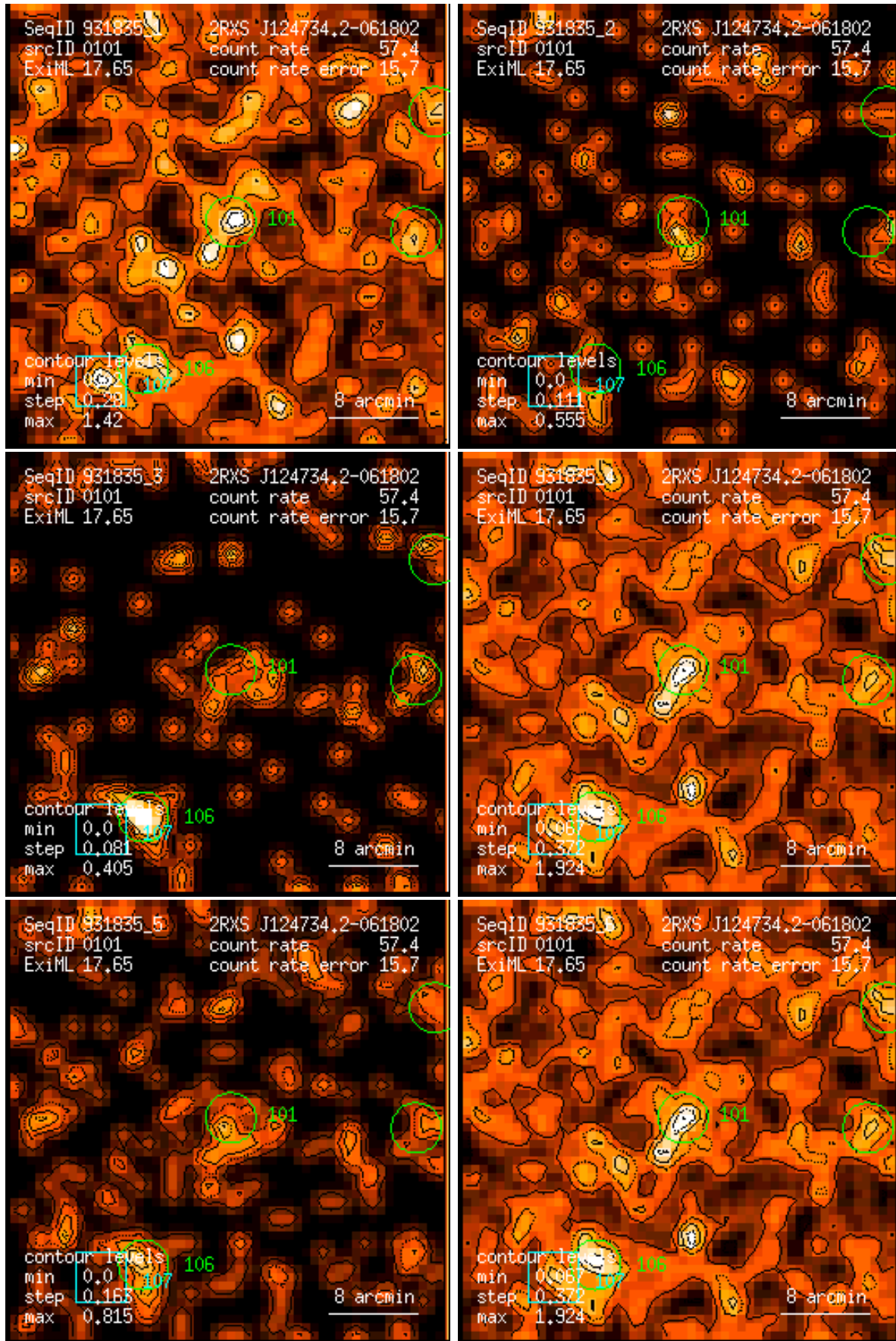
Figure 101: RASS 931835: detection 0101: band rate images, Gaussian filter: (1) PSPC channels 11 – 41, (2) 52 – 90, (3) 91 – 201, (4) 11 – 235, (5) 52 – 201, (6) 11 – 201. Broad band rates in counts/ks. Band rate contour levels in counts/ks/arcmin 2 .
