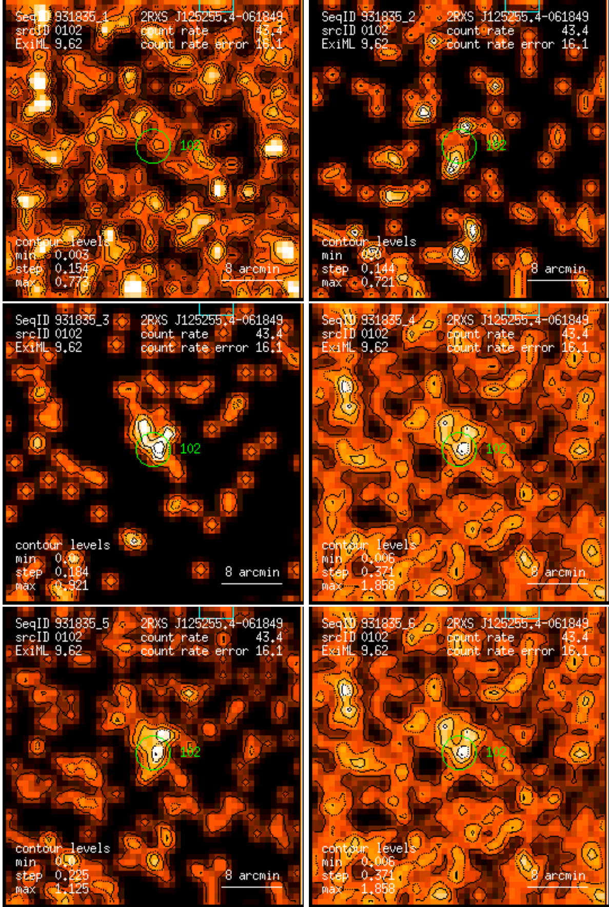
Figure 102: RASS 931835: detection 0102: band rate images, Gaussian filter: (1) PSPC channels 11 – 41, (2) 52 – 90, (3) 91 – 201, (4) 11 – 235, (5) 52 – 201, (6) 11 – 201. Broad band rates in counts/ks. Band rate contour levels in counts/ks/arcmin 2 .
