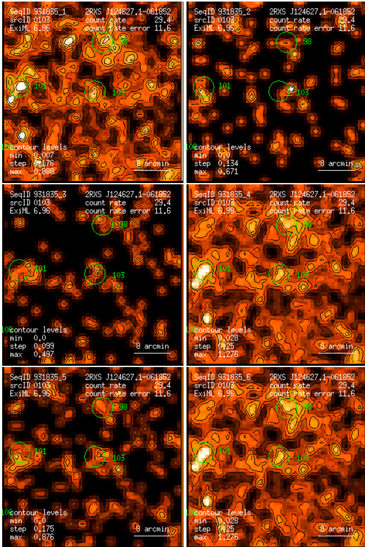
Figure 103: RASS 931835: detection 0103: band rate images, Gaussian filter: (1) PSPC channels 11 – 41, (2) 52 – 90, (3) 91 – 201, (4) 11 – 235, (5) 52 – 201, (6) 11 – 201. Broad band rates in counts/ks. Band rate contour levels in counts/ks/arcmin 2 .
