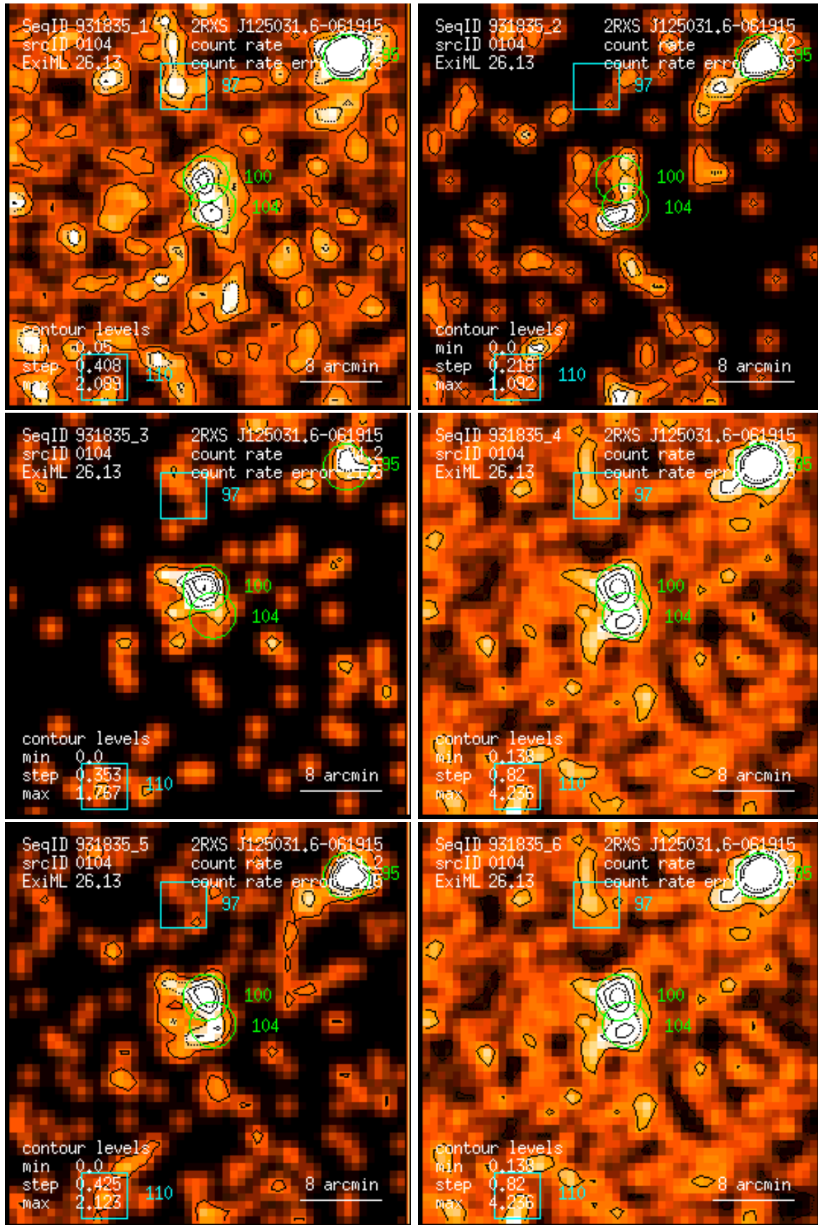
Figure 104: RASS 931835: detection 0104: band rate images, Gaussian filter: (1) PSPC channels 11 – 41, (2) 52 – 90, (3) 91 – 201, (4) 11 – 235, (5) 52 – 201, (6) 11 – 201. Broad band rates in counts/ks. Band rate contour levels in counts/ks/arcmin 2 .
