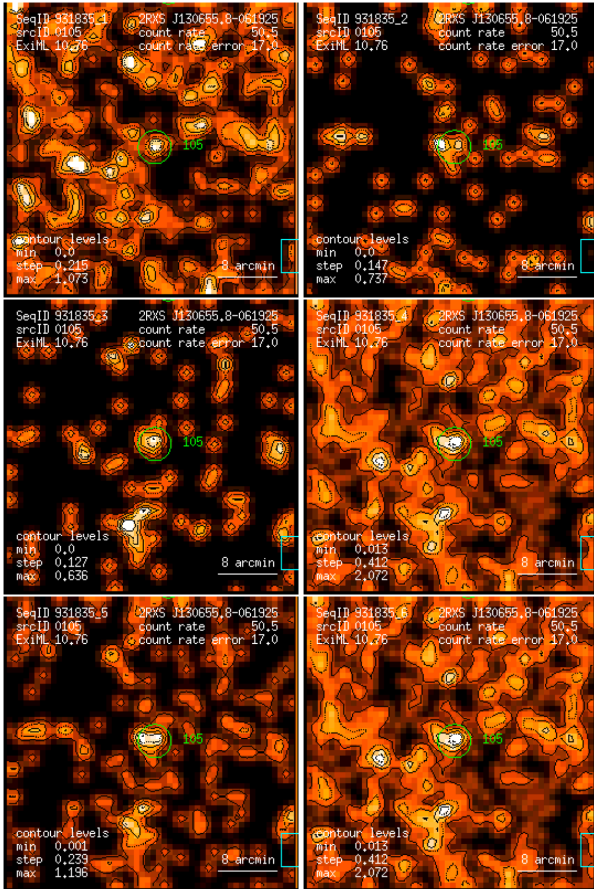
Figure 105: RASS 931835: detection 0105: band rate images, Gaussian filter: (1) PSPC channels 11 – 41, (2) 52 – 90, (3) 91 – 201, (4) 11 – 235, (5) 52 – 201, (6) 11 – 201. Broad band rates in counts/ks. Band rate contour levels in counts/ks/arcmin 2 .
