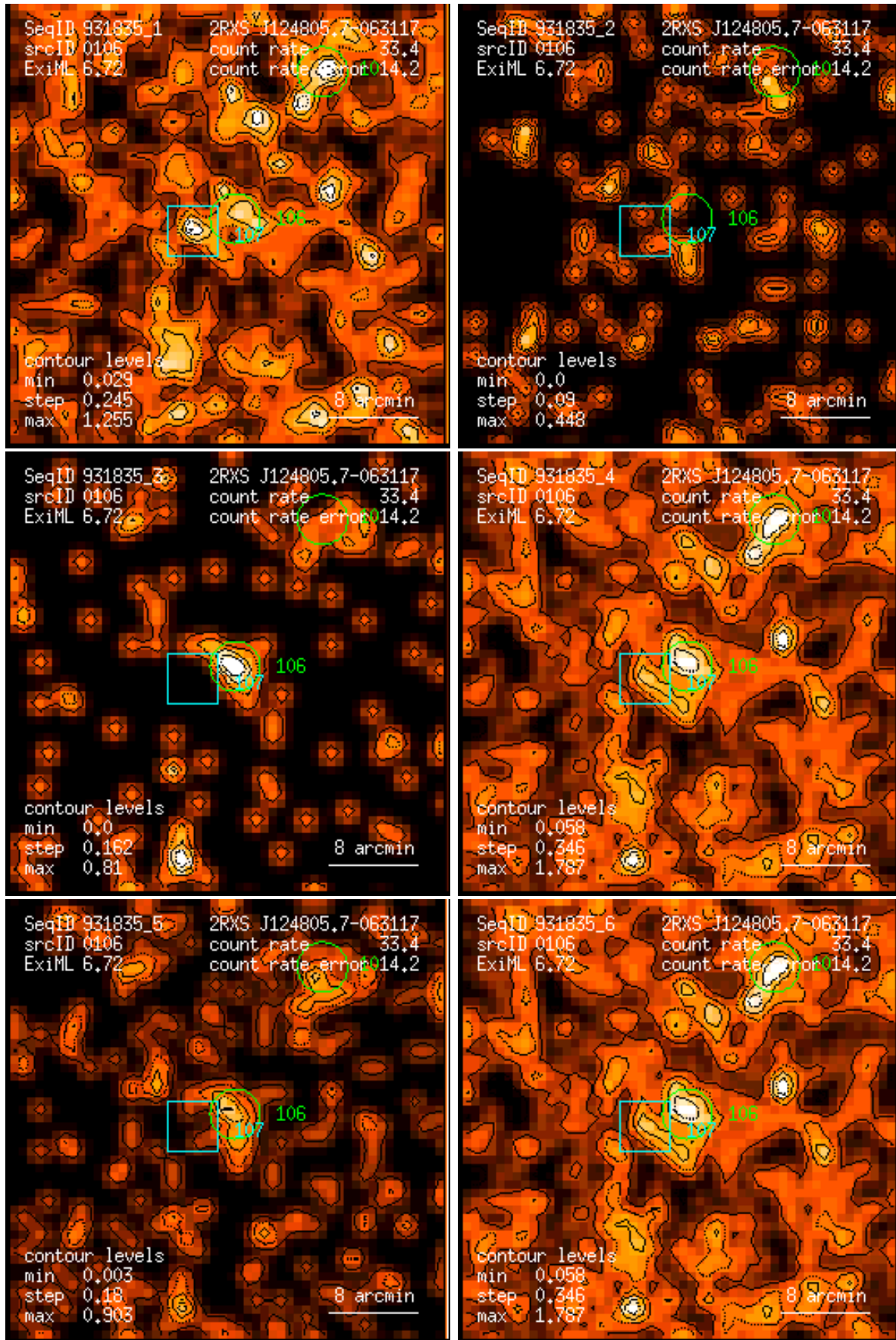
Figure 106: RASS 931835: detection 0106: band rate images, Gaussian filter: (1) PSPC channels 11 – 41, (2) 52 – 90, (3) 91 – 201, (4) 11 – 235, (5) 52 – 201, (6) 11 – 201. Broad band rates in counts/ks. Band rate contour levels in counts/ks/arcmin 2 .
