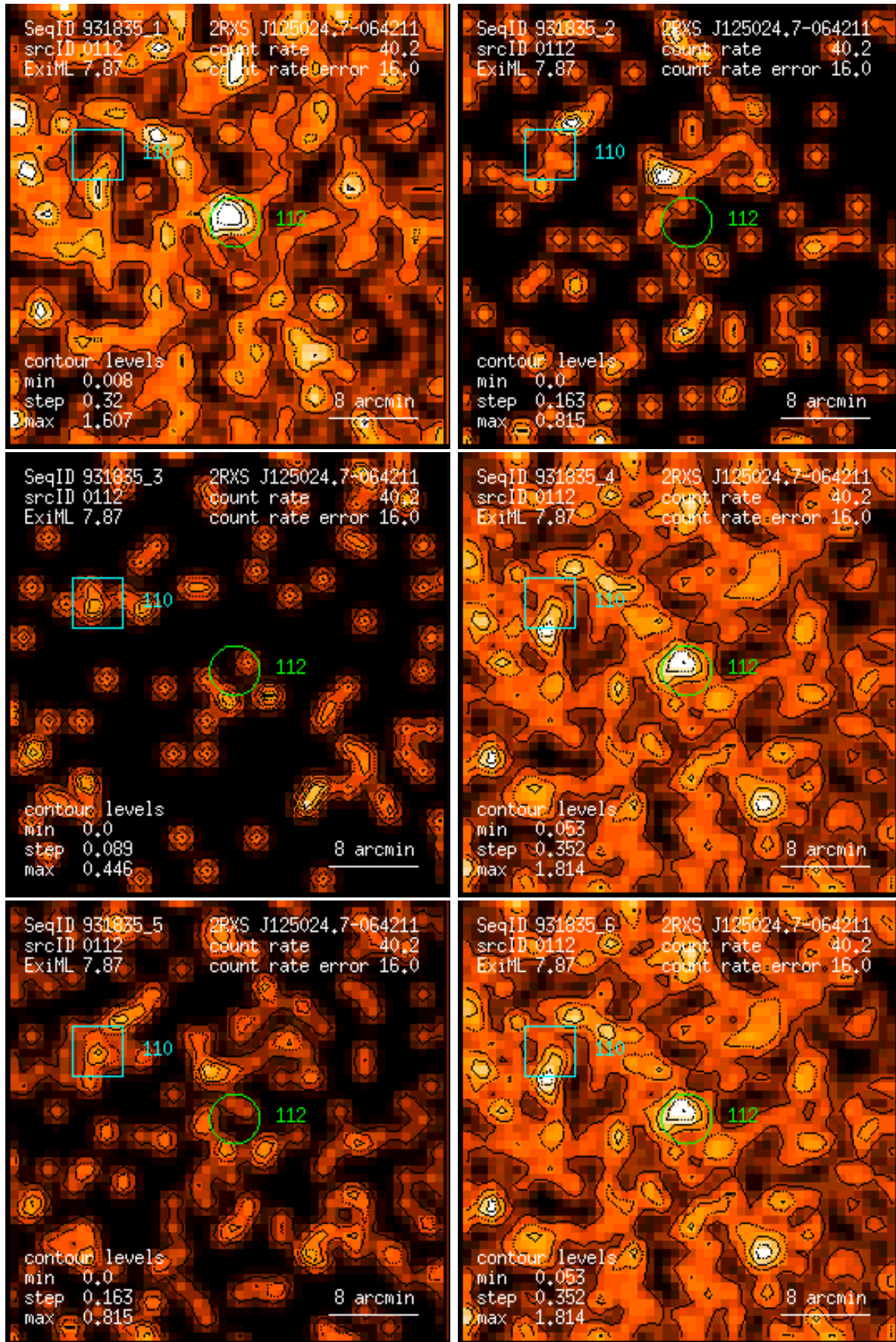
Figure 112: RASS 931835: detection 0112: band rate images, Gaussian filter: (1) PSPC channels 11 – 41, (2) 52 – 90, (3) 91 – 201, (4) 11 – 235, (5) 52 – 201, (6) 11 – 201. Broad band rates in counts/ks. Band rate contour levels in counts/ks/arcmin 2 .
