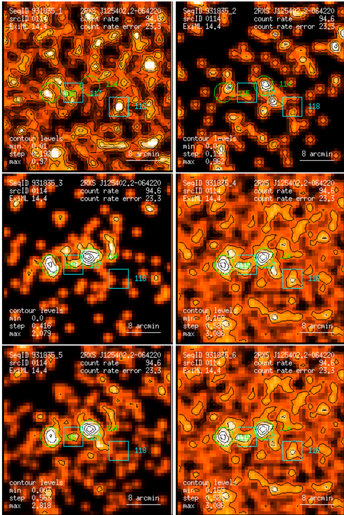
Figure 114: RASS 931835: detection 0114: band rate images, Gaussian filter: (1) PSPC channels 11 – 41, (2) 52 – 90, (3) 91 – 201, (4) 11 – 235, (5) 52 – 201, (6) 11 – 201. Broad band rates in counts/ks. Band rate contour levels in counts/ks/arcmin 2 .
