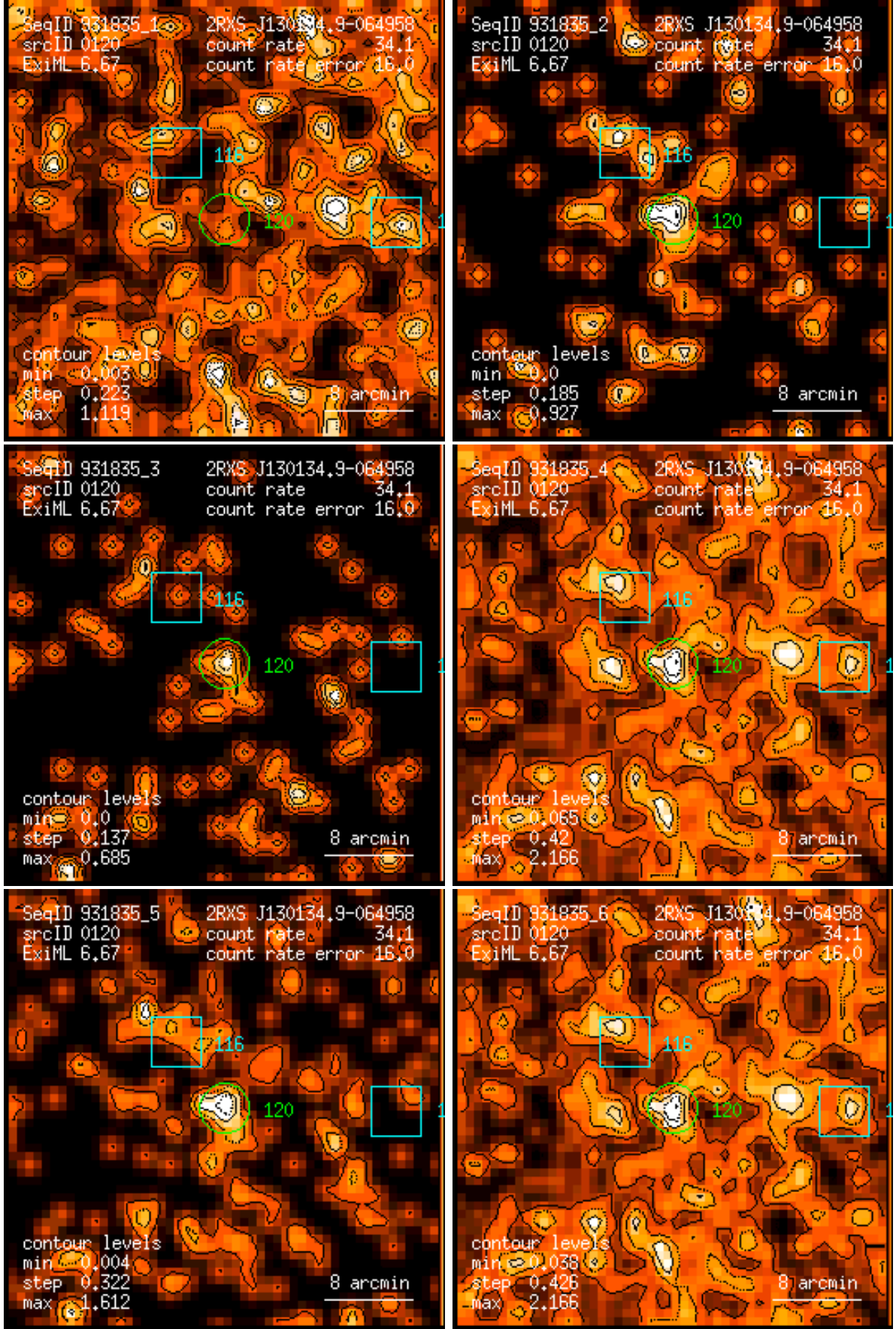
Figure 120: RASS 931835: detection 0120: band rate images, Gaussian filter: (1) PSPC channels 11 – 41, (2) 52 – 90, (3) 91 – 201, (4) 11 – 235, (5) 52 – 201, (6) 11 – 201. Broad band rates in counts/ks. Band rate contour levels in counts/ks/arcmin 2 .
