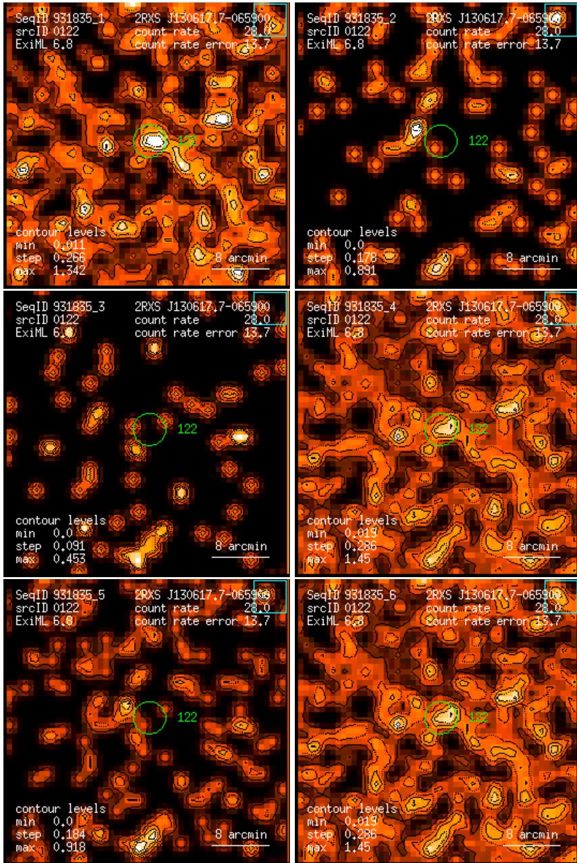
Figure 122: RASS 931835: detection 0122: band rate images, Gaussian filter: (1) PSPC channels 11 – 41, (2) 52 – 90, (3) 91 – 201, (4) 11 – 235, (5) 52 – 201, (6) 11 – 201. Broad band rates in counts/ks. Band rate contour levels in counts/ks/arcmin 2 .
