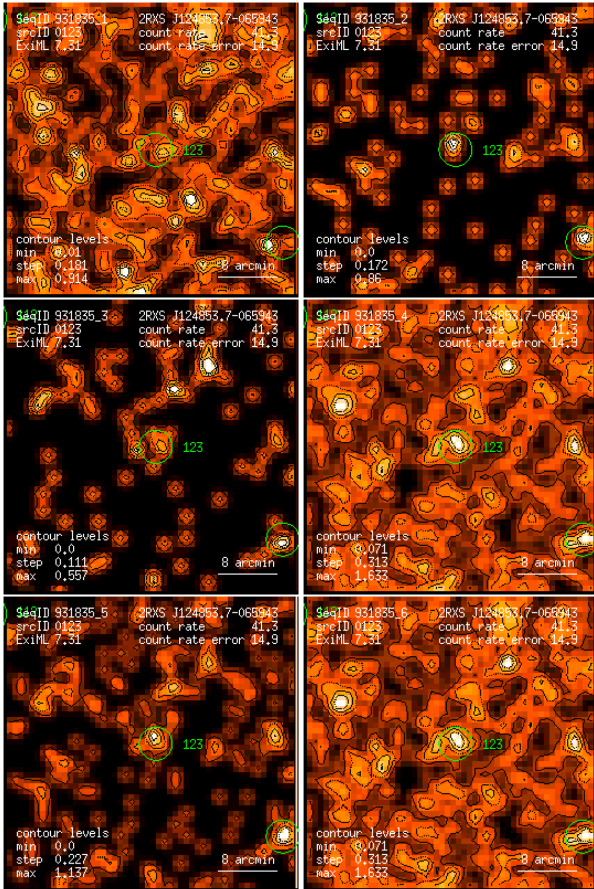
Figure 123: RASS 931835: detection 0123: band rate images, Gaussian filter: (1) PSPC channels 11 – 41, (2) 52 – 90, (3) 91 – 201, (4) 11 – 235, (5) 52 – 201, (6) 11 – 201. Broad band rates in counts/ks. Band rate contour levels in counts/ks/arcmin 2 .
