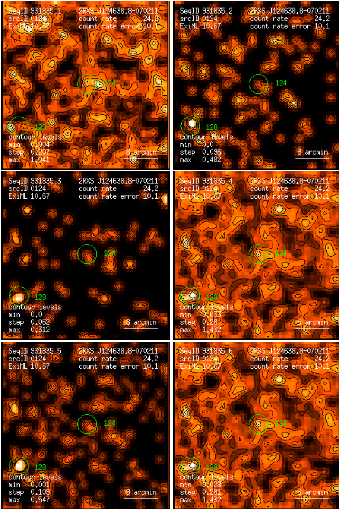
Figure 124: RASS 931835: detection 0124: band rate images, Gaussian filter: (1) PSPC channels 11 – 41, (2) 52 – 90, (3) 91 – 201, (4) 11 – 235, (5) 52 – 201, (6) 11 – 201. Broad band rates in counts/ks. Band rate contour levels in counts/ks/arcmin 2 .
