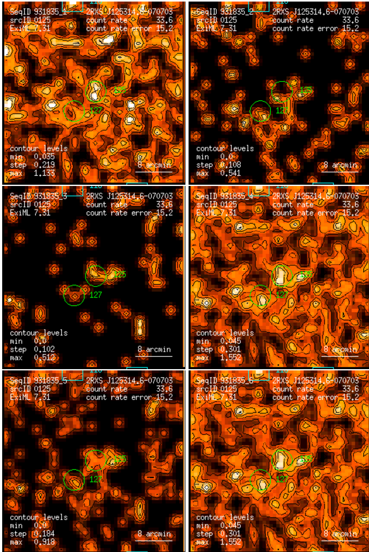
Figure 125: RASS 931835: detection 0125: band rate images, Gaussian filter: (1) PSPC channels 11 – 41, (2) 52 – 90, (3) 91 – 201, (4) 11 – 235, (5) 52 – 201, (6) 11 – 201. Broad band rates in counts/ks. Band rate contour levels in counts/ks/arcmin 2 .
