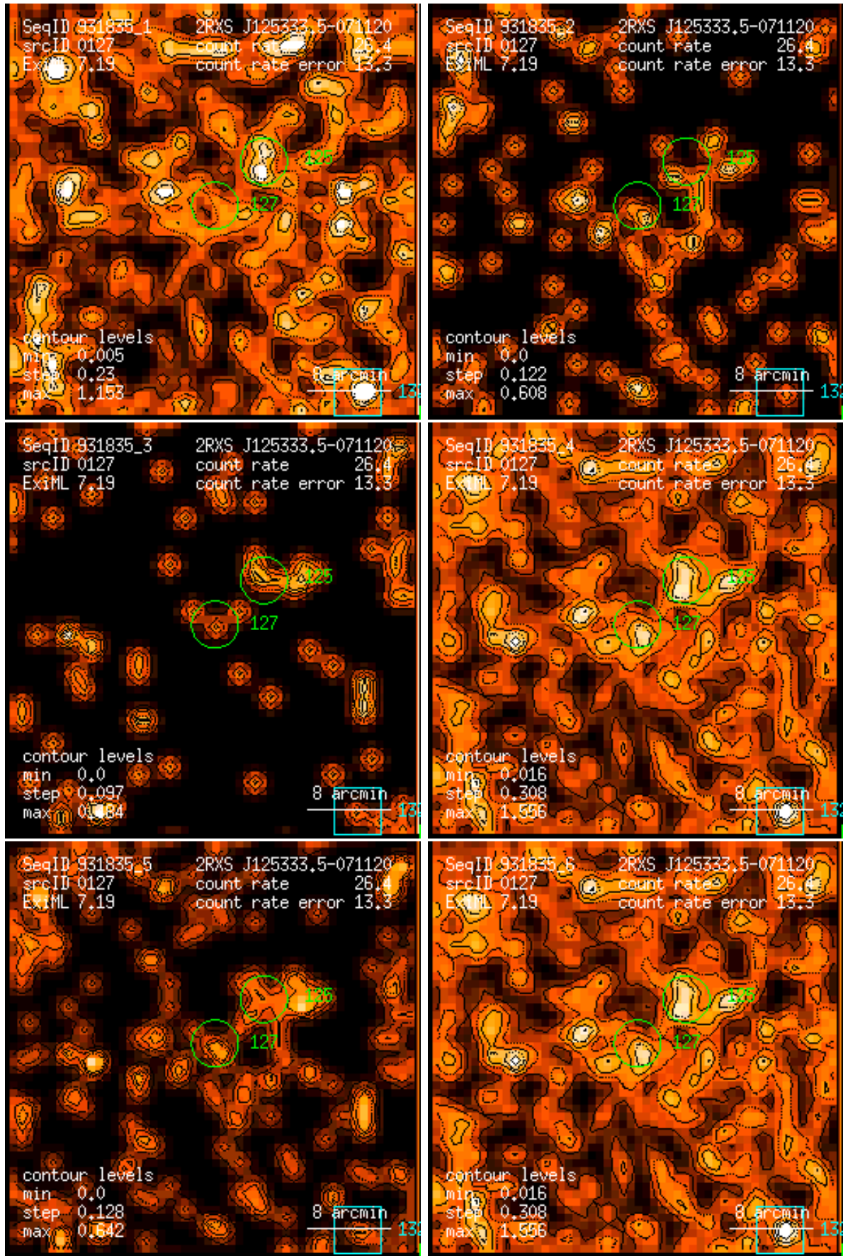
Figure 127: RASS 931835: detection 0127: band rate images, Gaussian filter: (1) PSPC channels 11 – 41, (2) 52 – 90, (3) 91 – 201, (4) 11 – 235, (5) 52 – 201, (6) 11 – 201. Broad band rates in counts/ks. Band rate contour levels in counts/ks/arcmin 2 .
