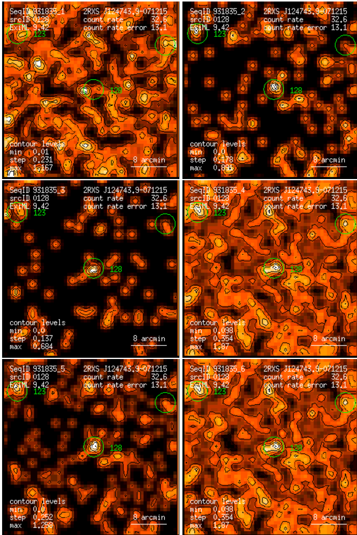
Figure 128: RASS 931835: detection 0128: band rate images, Gaussian filter: (1) PSPC channels 11 – 41, (2) 52 – 90, (3) 91 – 201, (4) 11 – 235, (5) 52 – 201, (6) 11 – 201. Broad band rates in counts/ks. Band rate contour levels in counts/ks/arcmin 2 .
