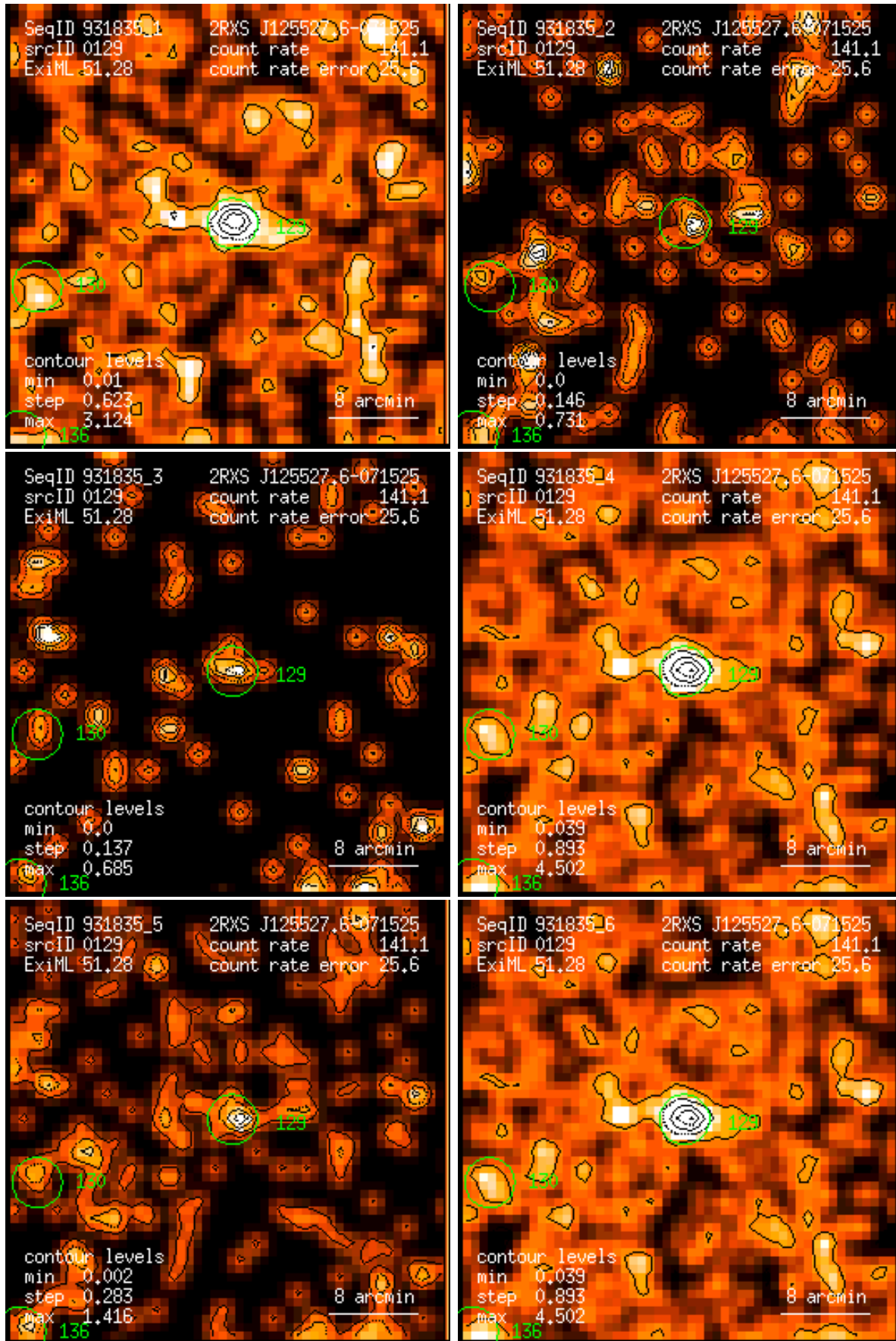
Figure 129: RASS 931835: detection 0129: band rate images, Gaussian filter: (1) PSPC channels 11 – 41, (2) 52 – 90, (3) 91 – 201, (4) 11 – 235, (5) 52 – 201, (6) 11 – 201. Broad band rates in counts/ks. Band rate contour levels in counts/ks/arcmin 2 .
