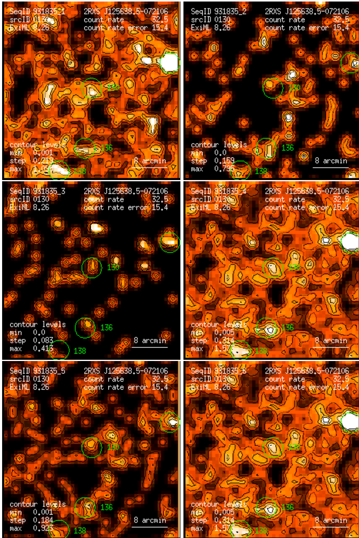
Figure 130: RASS 931835: detection 0130: band rate images, Gaussian filter: (1) PSPC channels 11 – 41, (2) 52 – 90, (3) 91 – 201, (4) 11 – 235, (5) 52 – 201, (6) 11 – 201. Broad band rates in counts/ks. Band rate contour levels in counts/ks/arcmin 2 .
