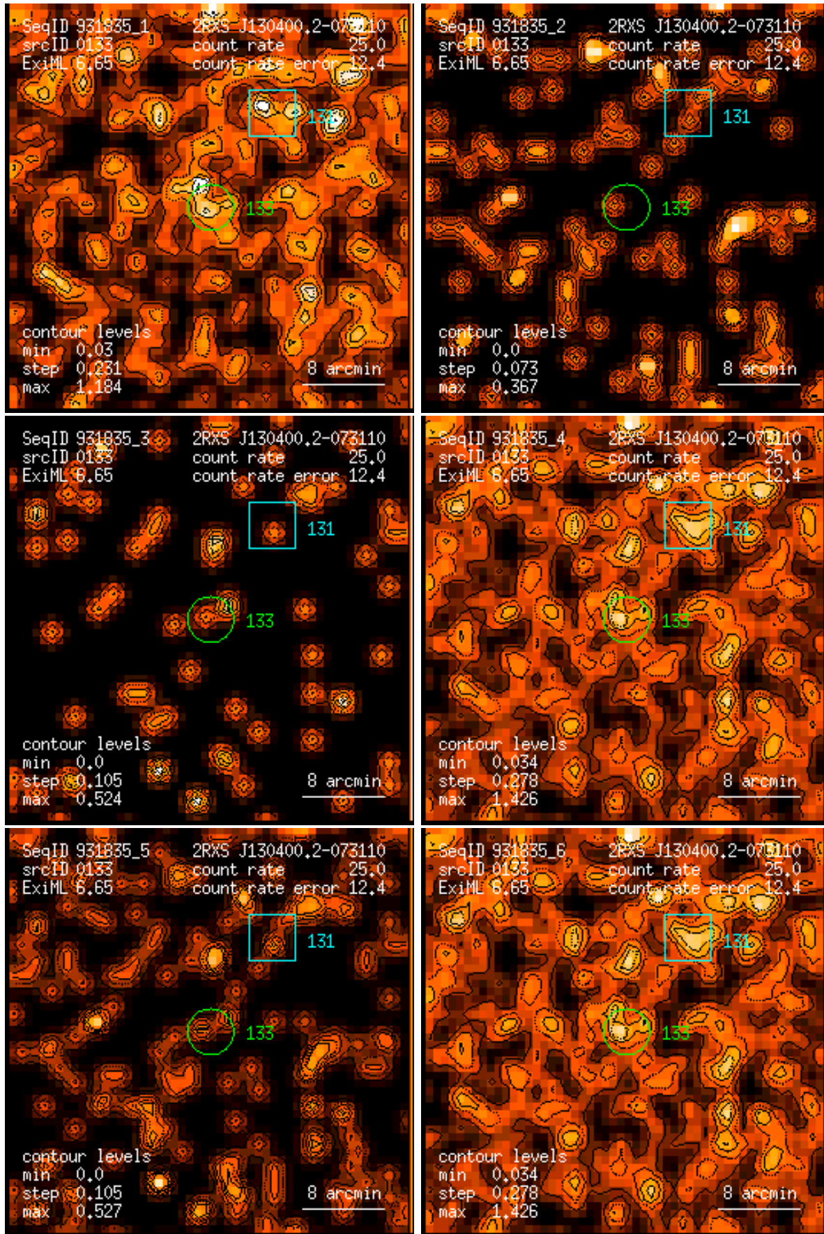
Figure 133: RASS 931835: detection 0133: band rate images, Gaussian filter: (1) PSPC channels 11 – 41, (2) 52 – 90, (3) 91 – 201, (4) 11 – 235, (5) 52 – 201, (6) 11 – 201. Broad band rates in counts/ks. Band rate contour levels in counts/ks/arcmin 2 .
