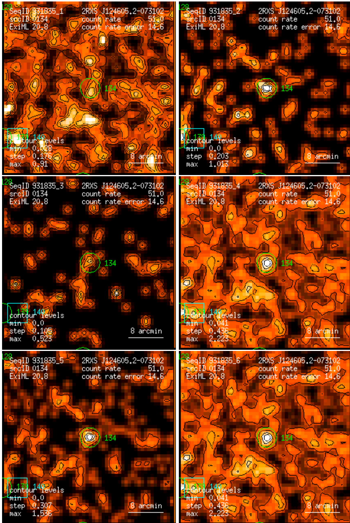
Figure 134: RASS 931835: detection 0134: band rate images, Gaussian filter: (1) PSPC channels 11 – 41, (2) 52 – 90, (3) 91 – 201, (4) 11 – 235, (5) 52 – 201, (6) 11 – 201. Broad band rates in counts/ks. Band rate contour levels in counts/ks/arcmin 2 .
