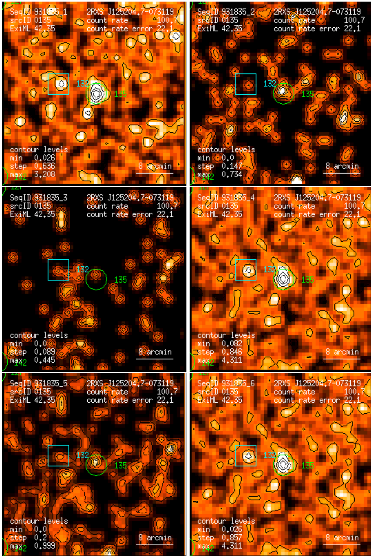
Figure 135: RASS 931835: detection 0135: band rate images, Gaussian filter: (1) PSPC channels 11 – 41, (2) 52 – 90, (3) 91 – 201, (4) 11 – 235, (5) 52 – 201, (6) 11 – 201. Broad band rates in counts/ks. Band rate contour levels in counts/ks/arcmin 2 .
