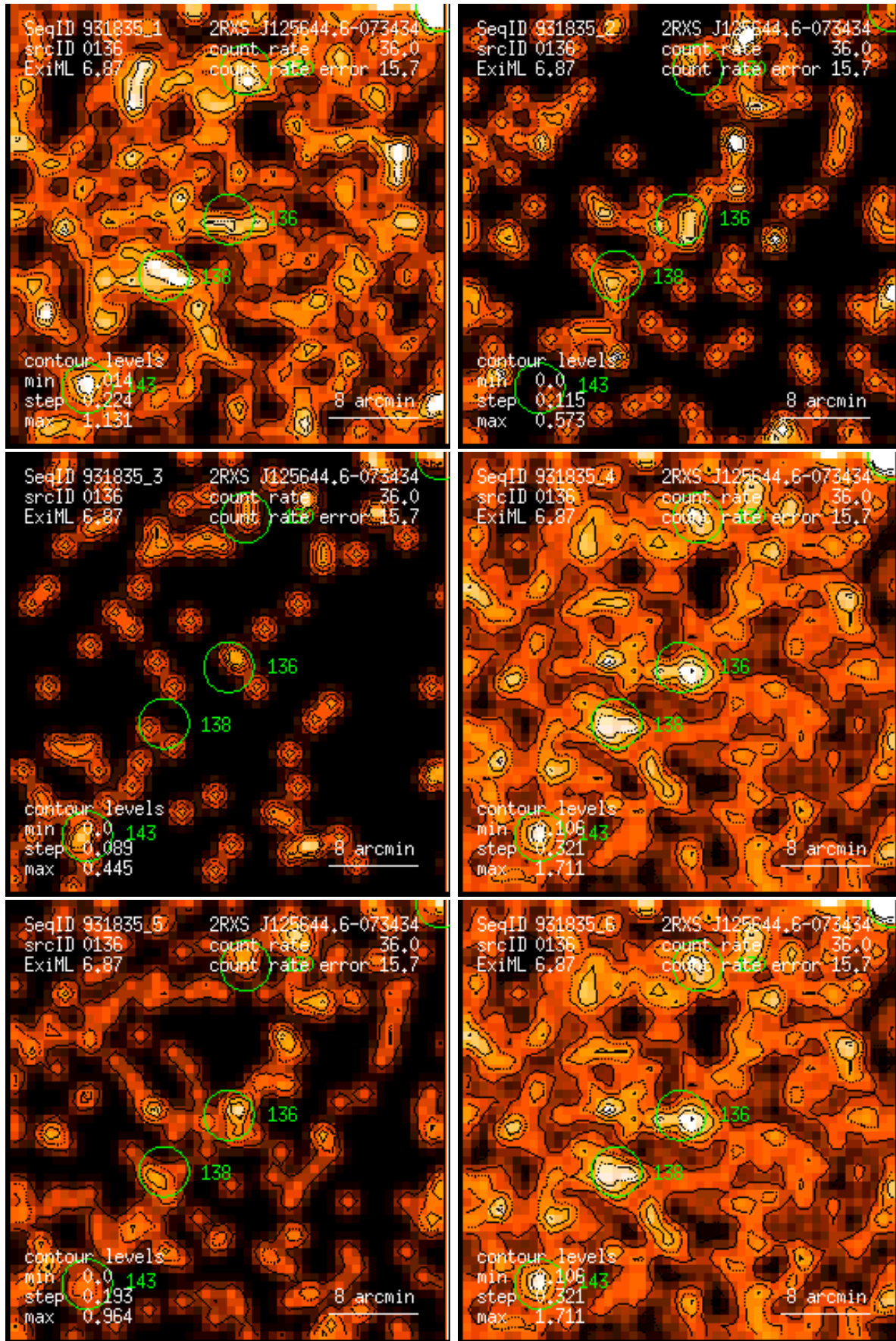
Figure 136: RASS 931835: detection 0136: band rate images, Gaussian filter: (1) PSPC channels 11 – 41, (2) 52 – 90, (3) 91 – 201, (4) 11 – 235, (5) 52 – 201, (6) 11 – 201. Broad band rates in counts/ks. Band rate contour levels in counts/ks/arcmin 2 .
