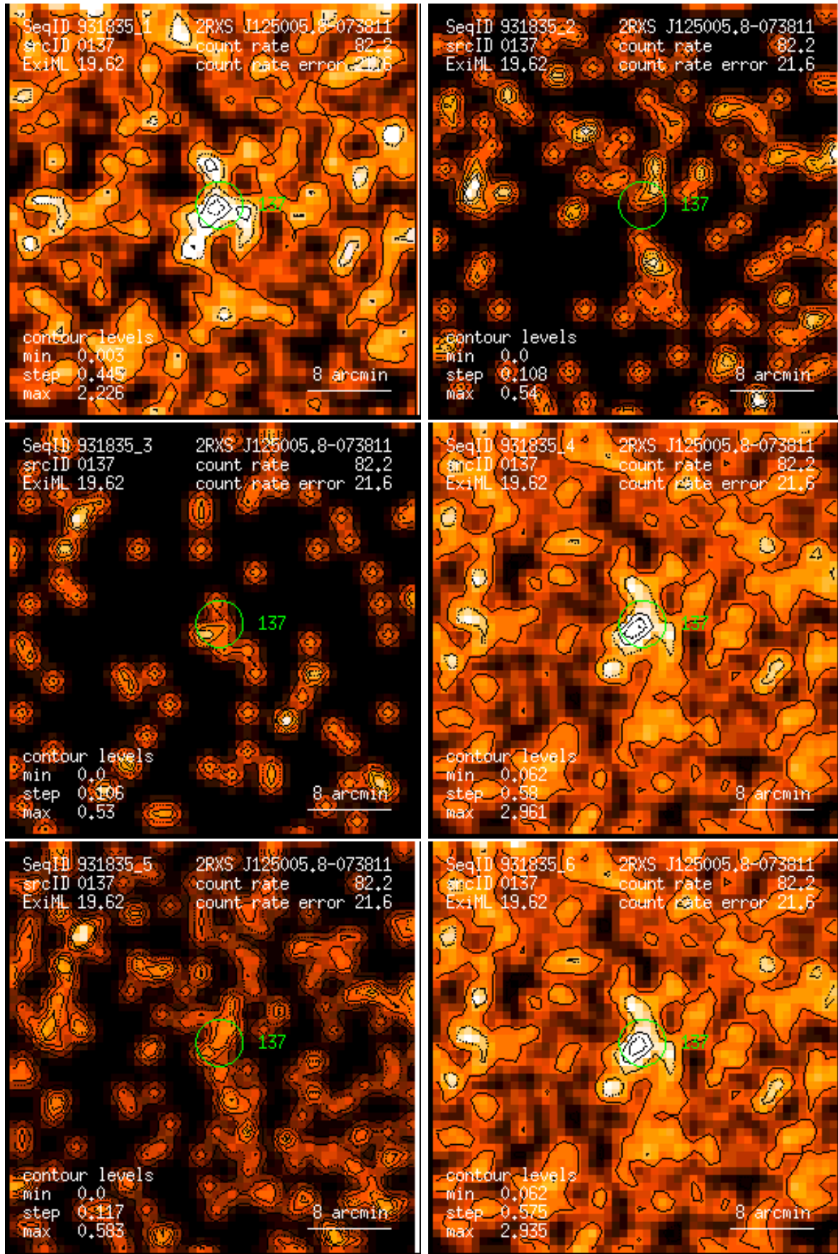
Figure 137: RASS 931835: detection 0137: band rate images, Gaussian filter: (1) PSPC channels 11 – 41, (2) 52 – 90, (3) 91 – 201, (4) 11 – 235, (5) 52 – 201, (6) 11 – 201. Broad band rates in counts/ks. Band rate contour levels in counts/ks/arcmin 2 .
