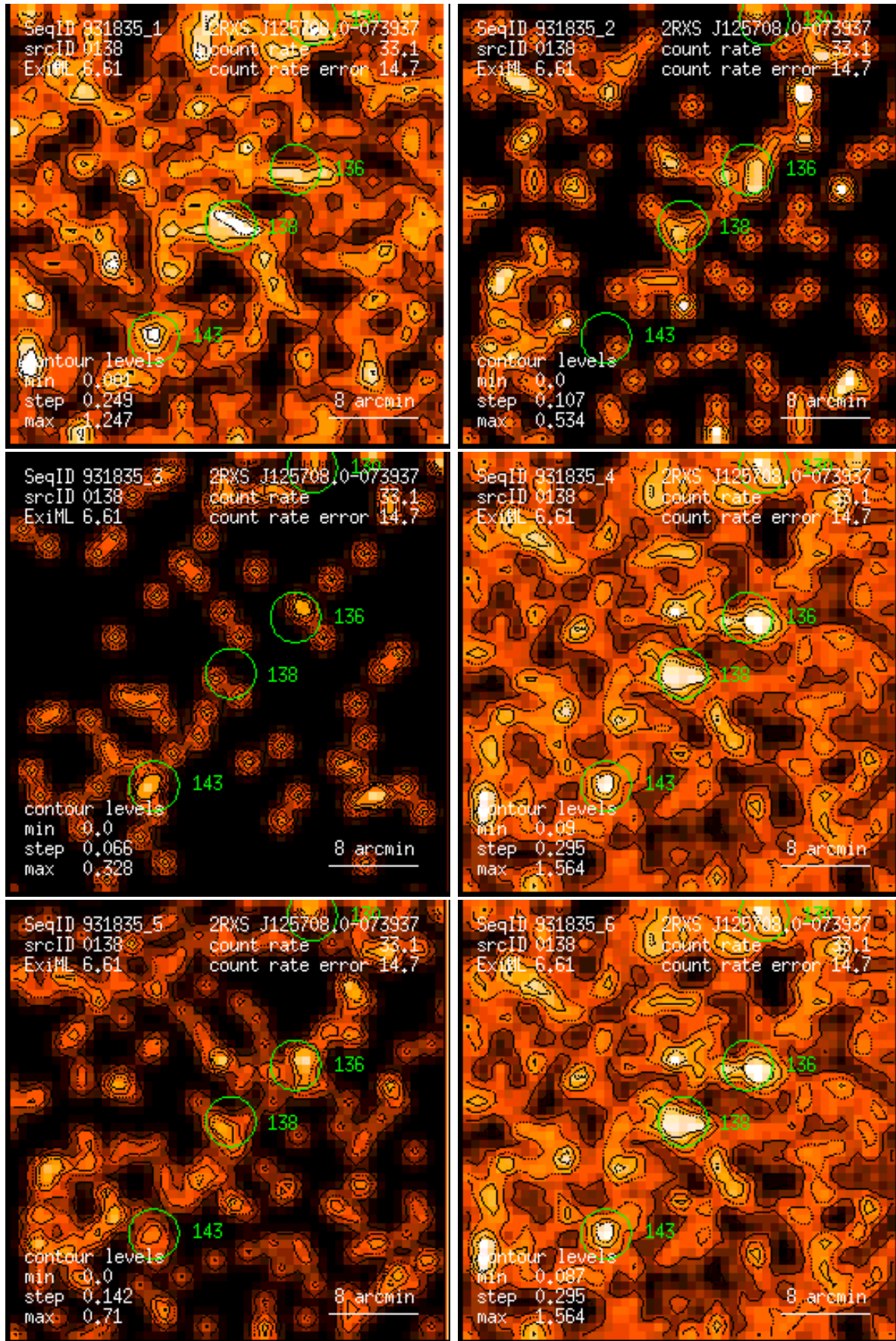
Figure 138: RASS 931835: detection 0138: band rate images, Gaussian filter: (1) PSPC channels 11 – 41, (2) 52 – 90, (3) 91 – 201, (4) 11 – 235, (5) 52 – 201, (6) 11 – 201. Broad band rates in counts/ks. Band rate contour levels in counts/ks/arcmin 2 .
