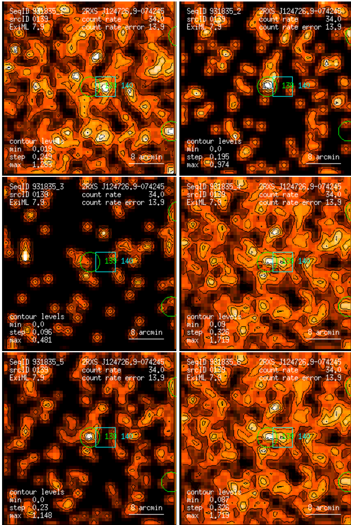
Figure 139: RASS 931835: detection 0139: band rate images, Gaussian filter: (1) PSPC channels 11 – 41, (2) 52 – 90, (3) 91 – 201, (4) 11 – 235, (5) 52 – 201, (6) 11 – 201. Broad band rates in counts/ks. Band rate contour levels in counts/ks/arcmin 2 .
