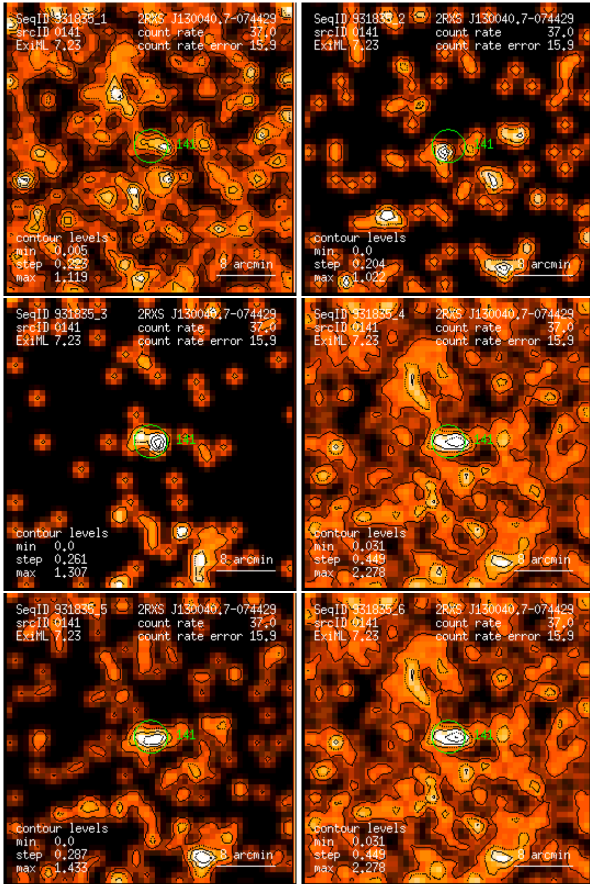
Figure 141: RASS 931835: detection 0141: band rate images, Gaussian filter: (1) PSPC channels 11 – 41, (2) 52 – 90, (3) 91 – 201, (4) 11 – 235, (5) 52 – 201, (6) 11 – 201. Broad band rates in counts/ks. Band rate contour levels in counts/ks/arcmin 2 .
