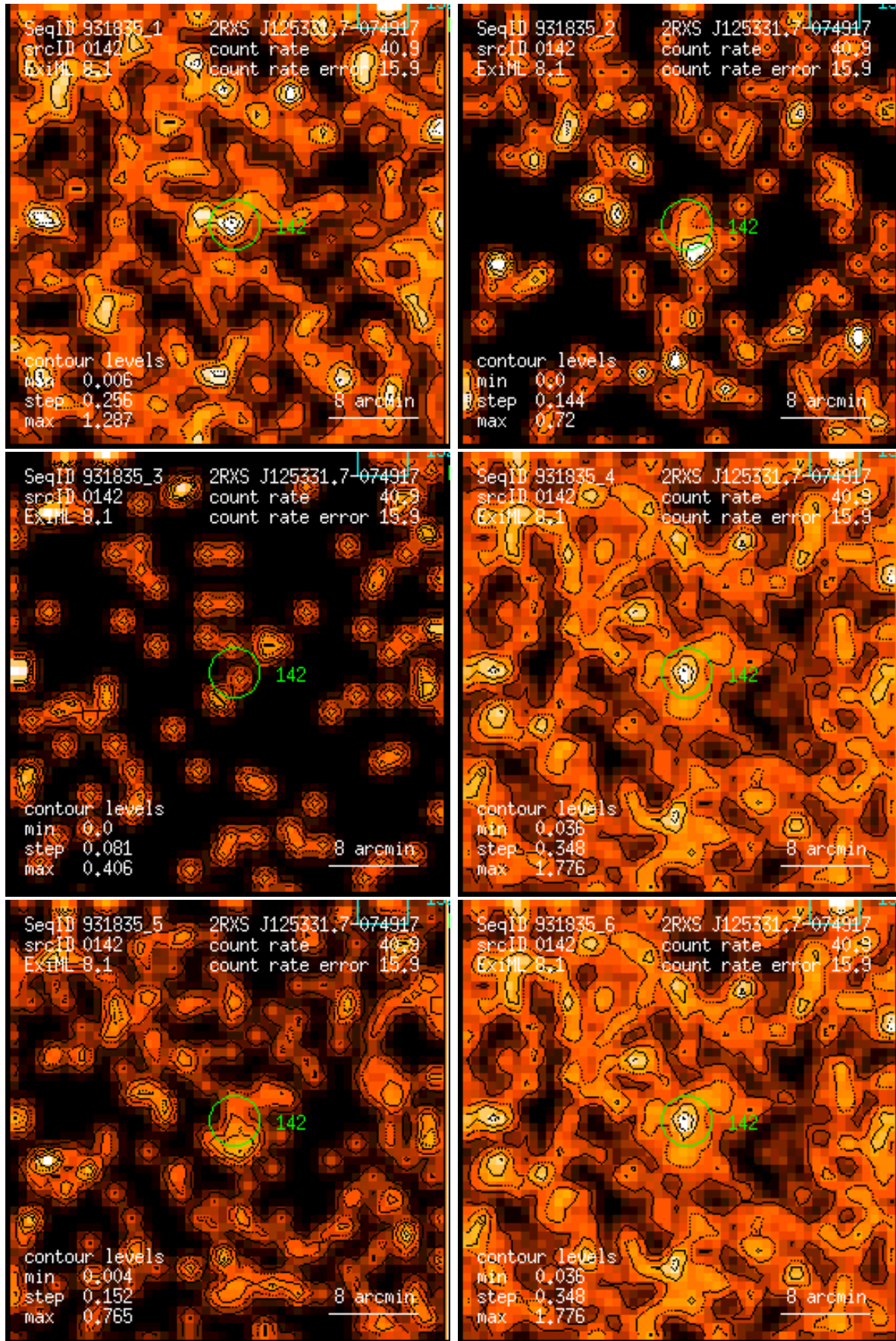
Figure 142: RASS 931835: detection 0142: band rate images, Gaussian filter: (1) PSPC channels 11 – 41, (2) 52 – 90, (3) 91 – 201, (4) 11 – 235, (5) 52 – 201, (6) 11 – 201. Broad band rates in counts/ks. Band rate contour levels in counts/ks/arcmin 2 .
