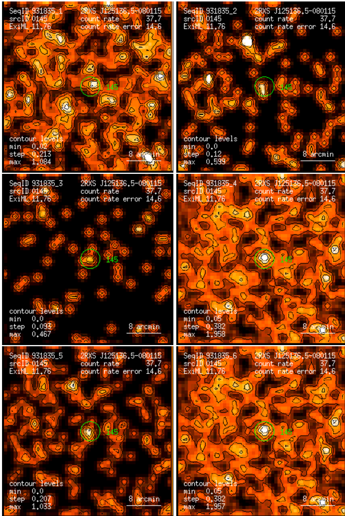
Figure 145: RASS 931835: detection 0145: band rate images, Gaussian filter: (1) PSPC channels 11 – 41, (2) 52 – 90, (3) 91 – 201, (4) 11 – 235, (5) 52 – 201, (6) 11 – 201. Broad band rates in counts/ks. Band rate contour levels in counts/ks/arcmin 2 .
