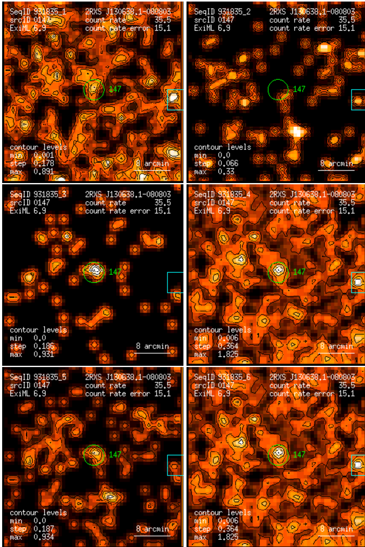
Figure 147: RASS 931835: detection 0147: band rate images, Gaussian filter: (1) PSPC channels 11 – 41, (2) 52 – 90, (3) 91 – 201, (4) 11 – 235, (5) 52 – 201, (6) 11 – 201. Broad band rates in counts/ks. Band rate contour levels in counts/ks/arcmin 2 .
