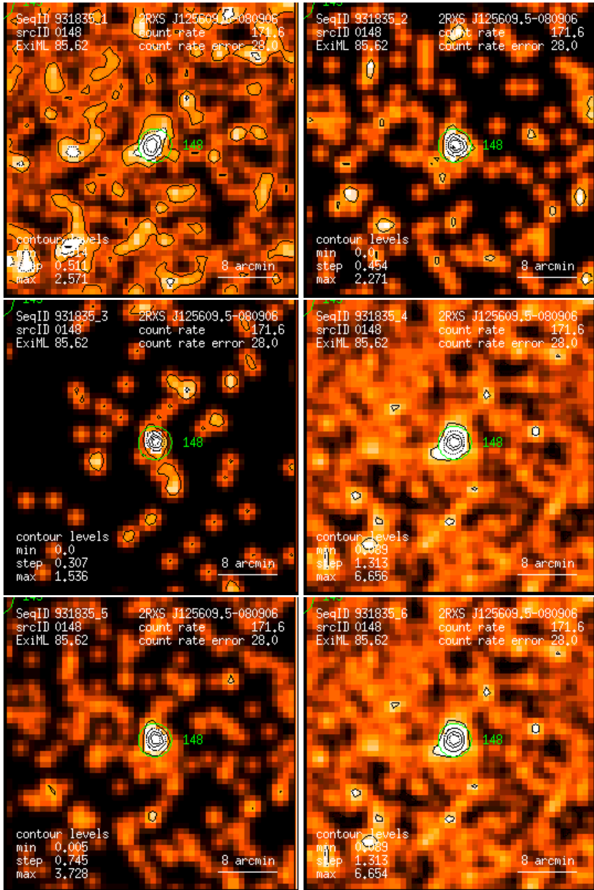
Figure 148: RASS 931835: detection 0148: band rate images, Gaussian filter: (1) PSPC channels 11 – 41, (2) 52 – 90, (3) 91 – 201, (4) 11 – 235, (5) 52 – 201, (6) 11 – 201. Broad band rates in counts/ks. Band rate contour levels in counts/ks/arcmin 2 .
