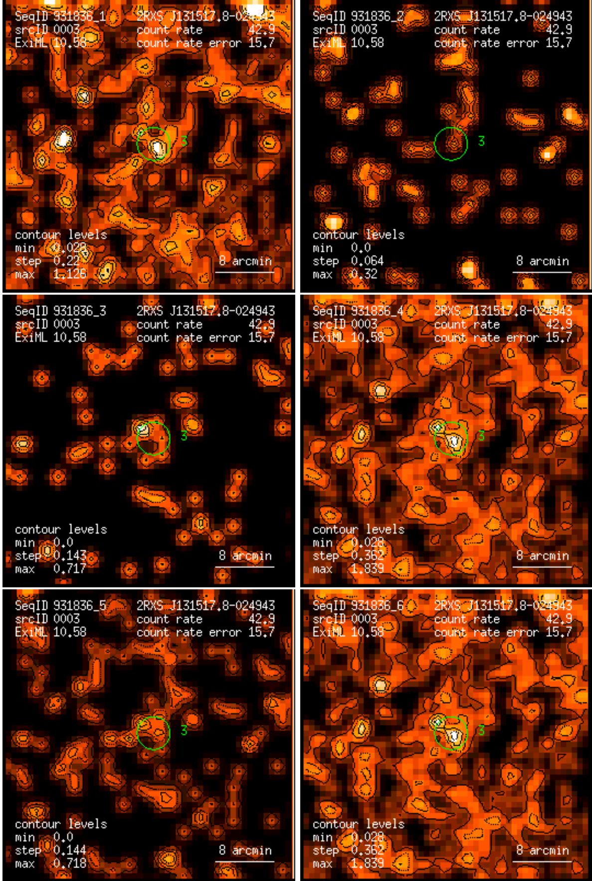
Figure 3: RASS 931836: detection 0003: band rate images, Gaussian filter: (1) PSPC channels 11 – 41, (2) 52 – 90, (3) 91 – 201, (4) 11 – 235, (5) 52 – 201, (6) 11 – 201. Broad band rates in counts/ks. Band rate contour levels in counts/ks/arcmin 2 .
