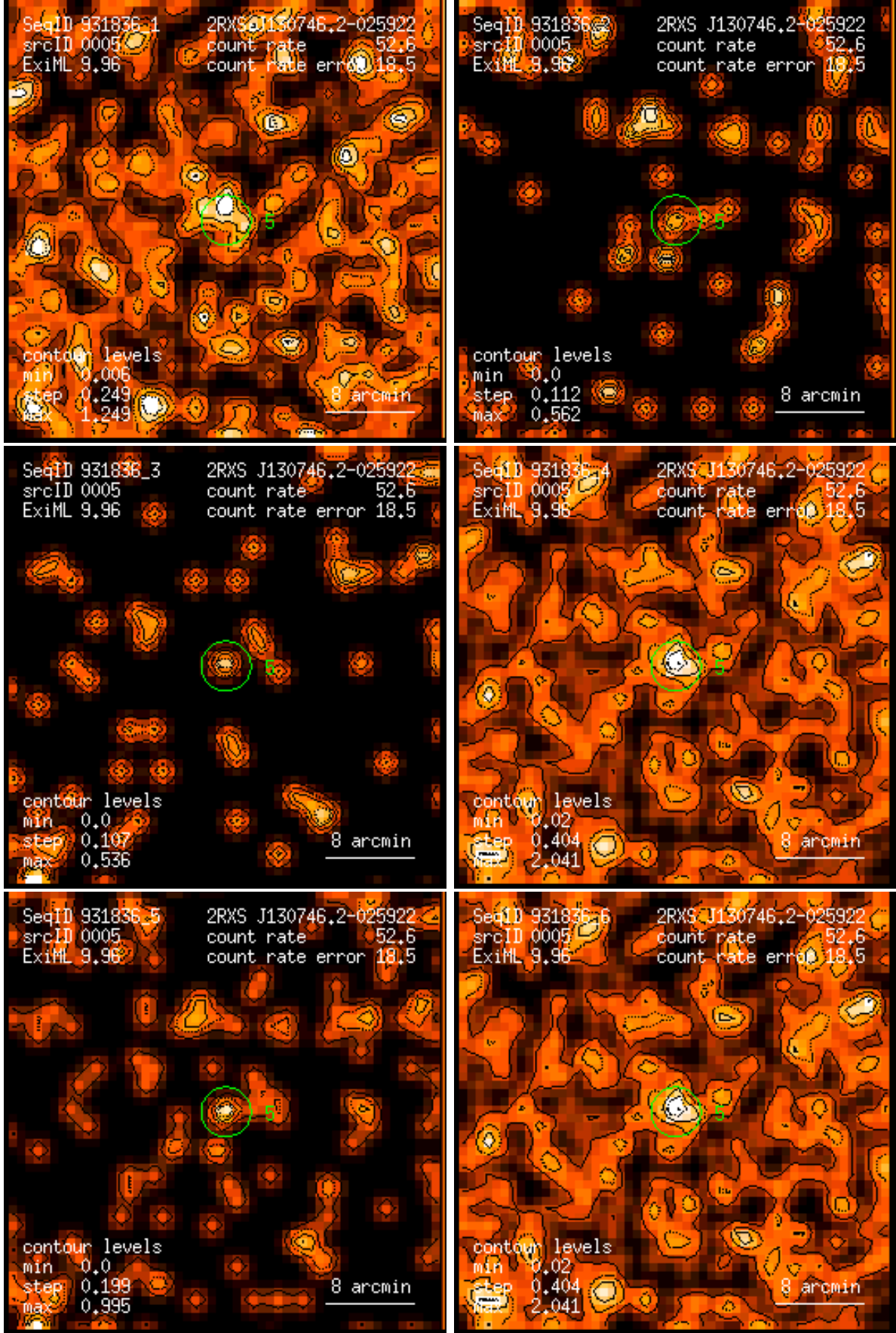
Figure 5: RASS 931836: detection 0005: band rate images, Gaussian filter: (1) PSPC channels 11 – 41, (2) 52 – 90, (3) 91 – 201, (4) 11 – 235, (5) 52 – 201, (6) 11 – 201. Broad band rates in counts/ks. Band rate contour levels in counts/ks/arcmin 2 .
