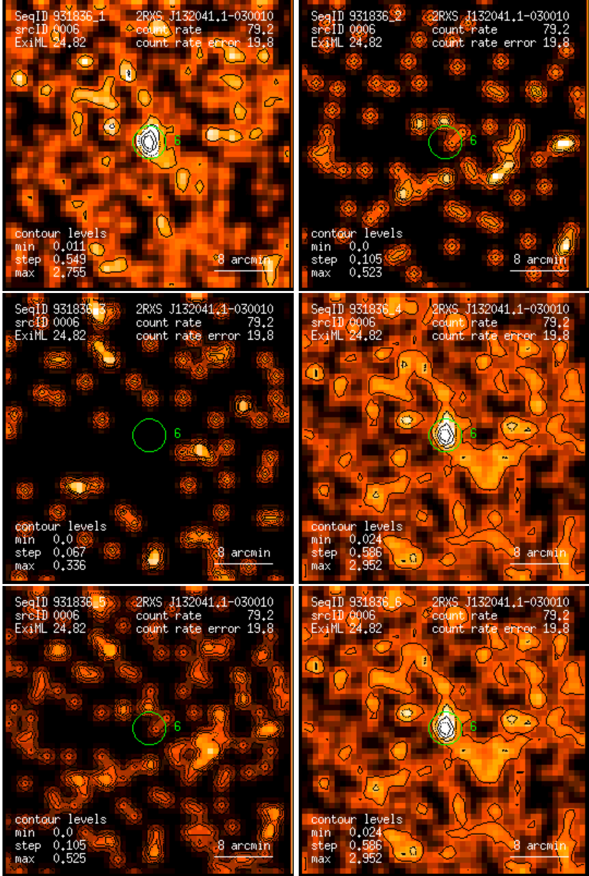
Figure 6: RASS 931836: detection 0006: band rate images, Gaussian filter: (1) PSPC channels 11 – 41, (2) 52 – 90, (3) 91 – 201, (4) 11 – 235, (5) 52 – 201, (6) 11 – 201. Broad band rates in counts/ks. Band rate contour levels in counts/ks/arcmin 2 .
