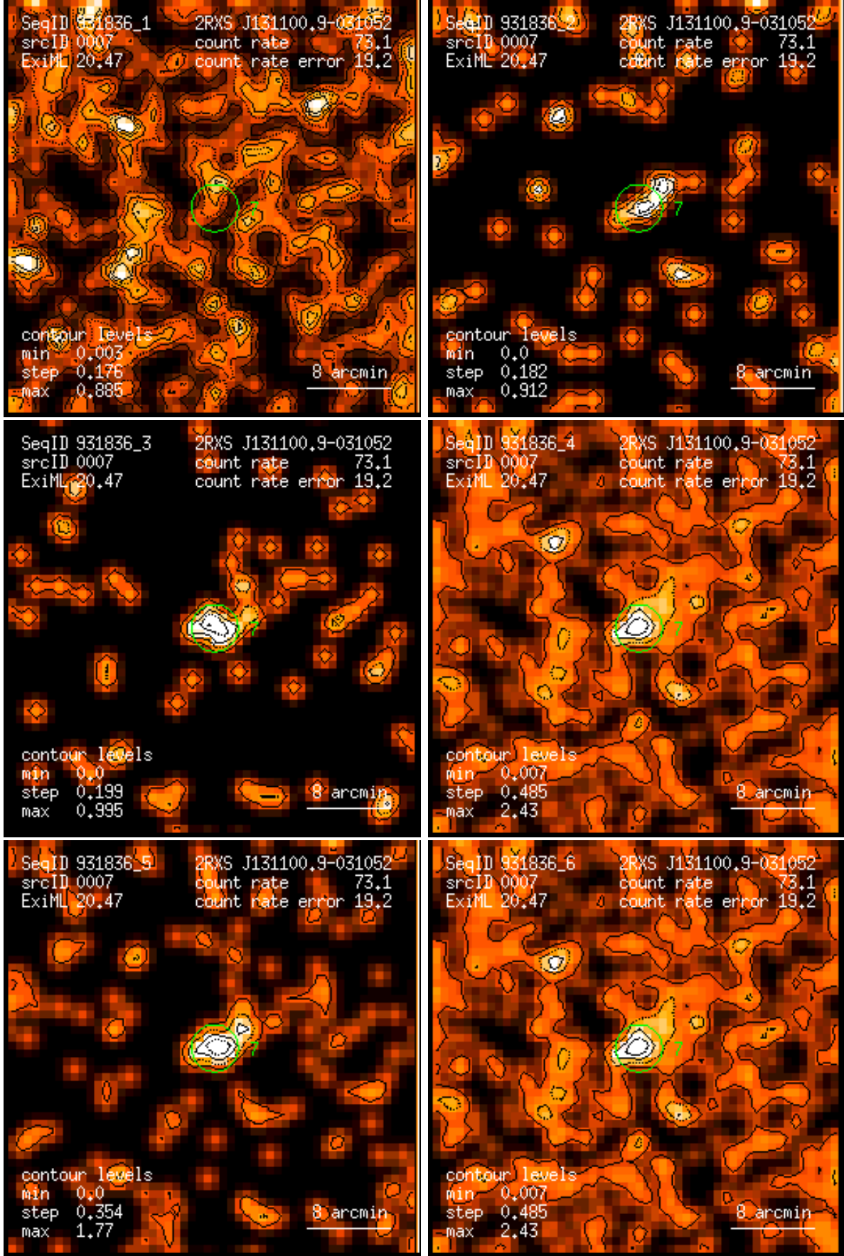
Figure 7: RASS 931836: detection 0007: band rate images, Gaussian filter: (1) PSPC channels 11 – 41, (2) 52 – 90, (3) 91 – 201, (4) 11 – 235, (5) 52 – 201, (6) 11 – 201. Broad band rates in counts/ks. Band rate contour levels in counts/ks/arcmin 2 .
