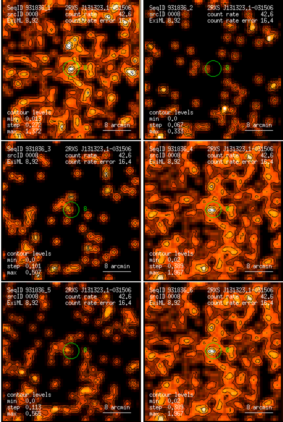
Figure 8: RASS 931836: detection 0008: band rate images, Gaussian filter: (1) PSPC channels 11 – 41, (2) 52 – 90, (3) 91 – 201, (4) 11 – 235, (5) 52 – 201, (6) 11 – 201. Broad band rates in counts/ks. Band rate contour levels in counts/ks/arcmin 2 .
