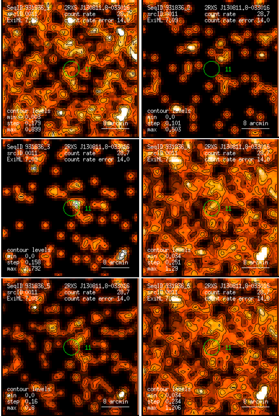
Figure 11: RASS 931836: detection 0011: band rate images, Gaussian filter: (1) PSPC channels 11 – 41, (2) 52 – 90, (3) 91 – 201, (4) 11 – 235, (5) 52 – 201, (6) 11 – 201. Broad band rates in counts/ks. Band rate contour levels in counts/ks/arcmin 2 .
