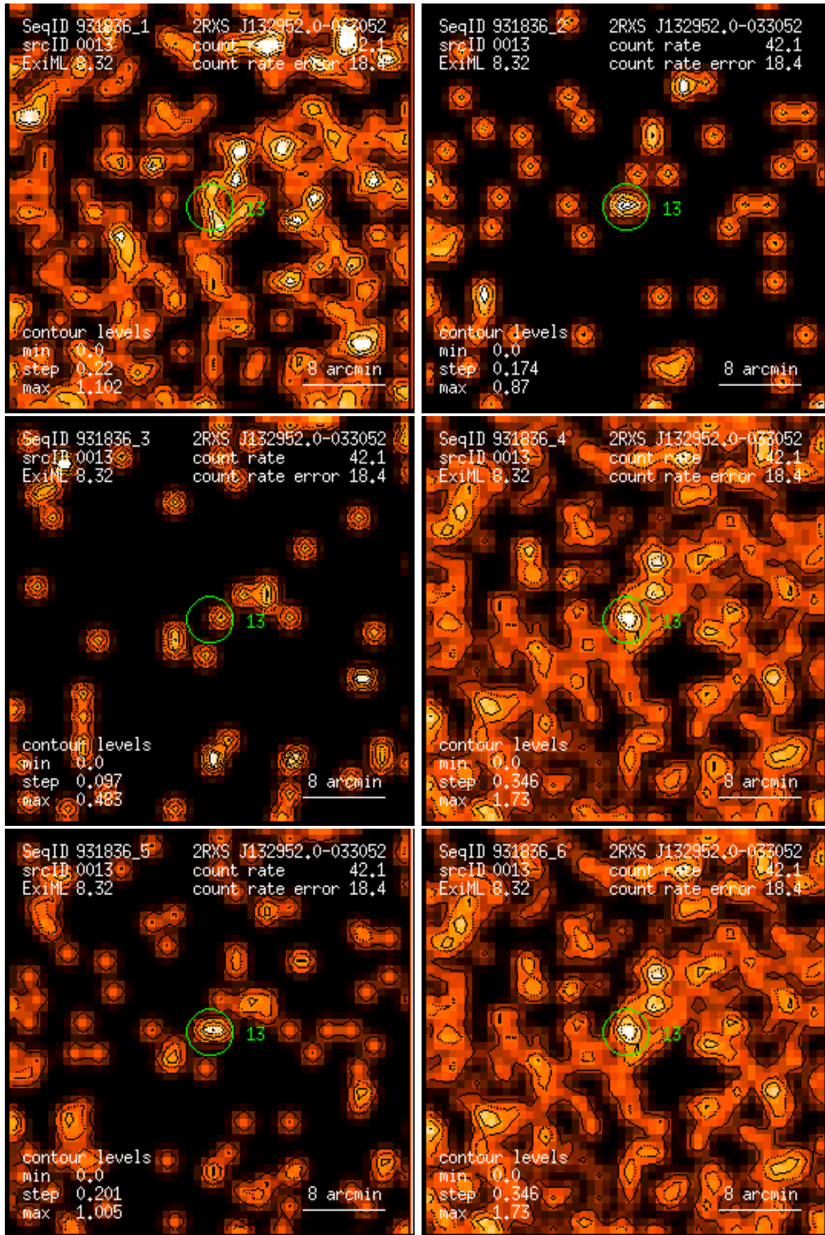
Figure 13: RASS 931836: detection 0013: band rate images, Gaussian filter: (1) PSPC channels 11 – 41, (2) 52 – 90, (3) 91 – 201, (4) 11 – 235, (5) 52 – 201, (6) 11 – 201. Broad band rates in counts/ks. Band rate contour levels in counts/ks/arcmin 2 .
