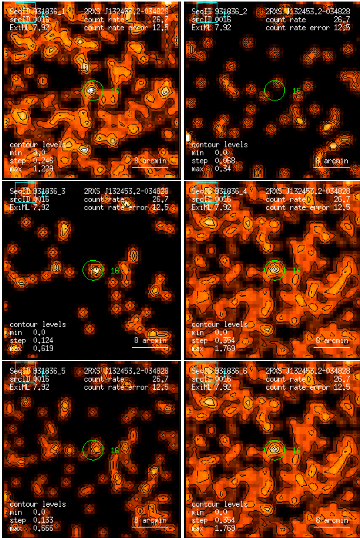
Figure 16: RASS 931836: detection 0016: band rate images, Gaussian filter: (1) PSPC channels 11 – 41, (2) 52 – 90, (3) 91 – 201, (4) 11 – 235, (5) 52 – 201, (6) 11 – 201. Broad band rates in counts/ks. Band rate contour levels in counts/ks/arcmin 2 .
