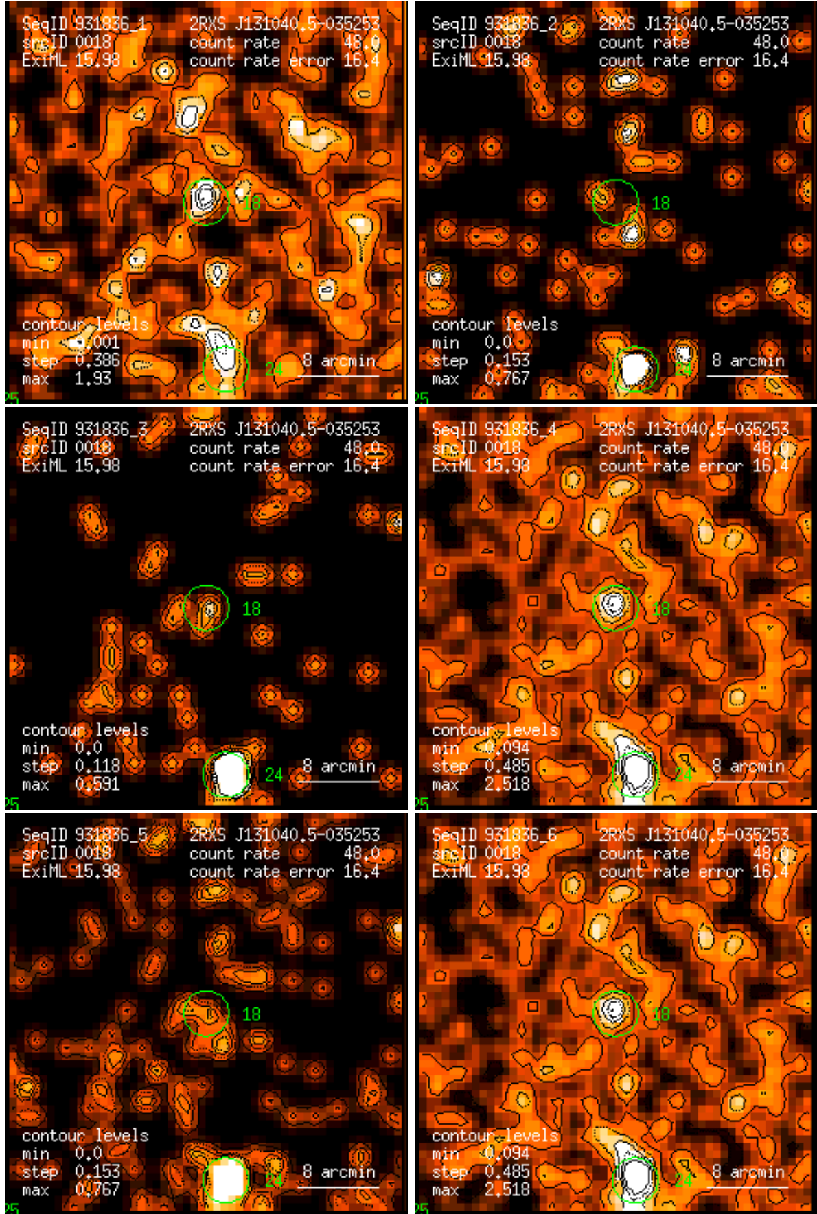
Figure 18: RASS 931836: detection 0018: band rate images, Gaussian filter: (1) PSPC channels 11 – 41, (2) 52 – 90, (3) 91 – 201, (4) 11 – 235, (5) 52 – 201, (6) 11 – 201. Broad band rates in counts/ks. Band rate contour levels in counts/ks/arcmin 2 .
